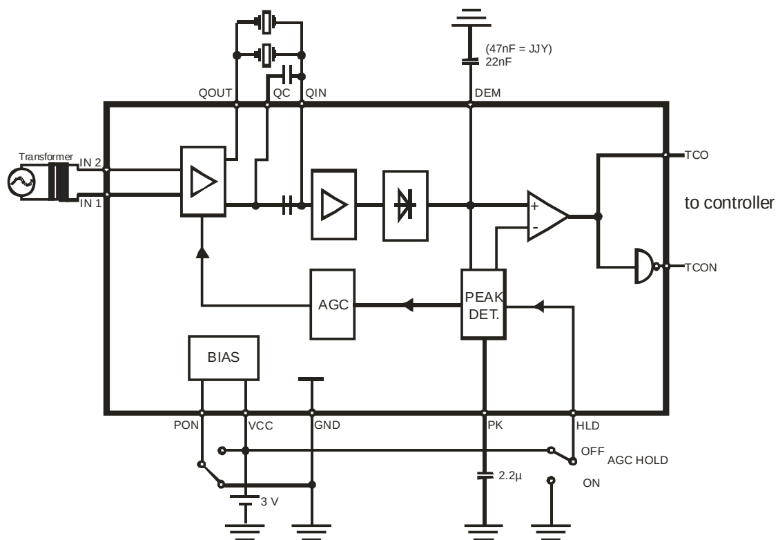
Figure 13. Test circuit
