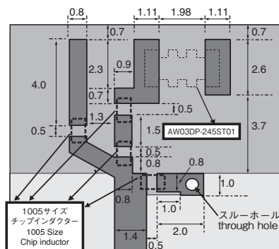
電極パターン(基板表面): AW03DP-245ST01*[特許申請中] Land pattern (Surface of the Substrate) [Patent Pending]
