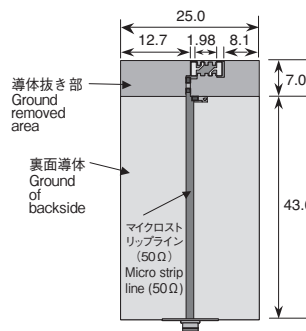
基板全体図(基板表面): AM03DP-ST01* Evaluated board (Surface of the Substrate)
