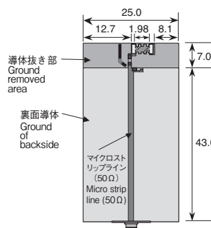
基板全体図(基板表面): AW03DP-245ST01* Evaluated board (Surface of the Substrate)
