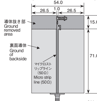
基板全体図(基板表面): AM11DP-ST01* Evaluated board (Surface of the Substrate)
