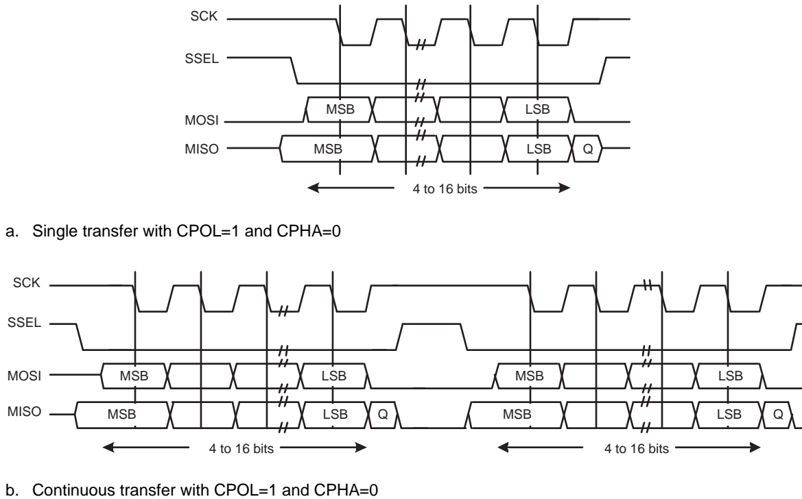
Fig 39. SPI frame format with CPOL = 1 and CPHA = 0 (a) Single and b) Continuous Transfer)
