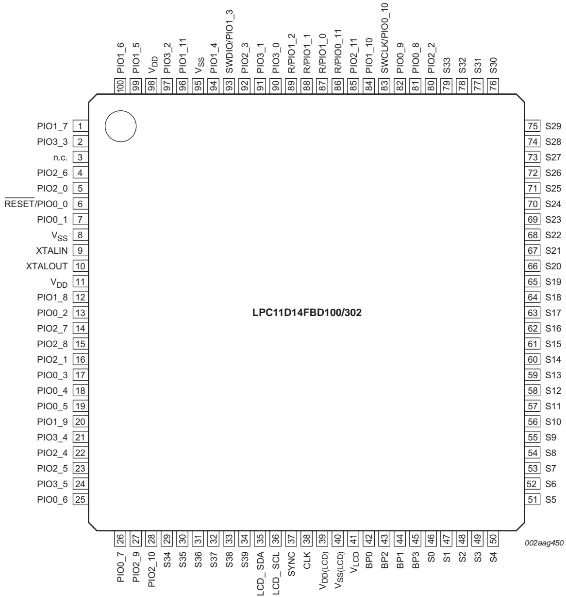
Fig 21. Pin configuration LQFP100 package
