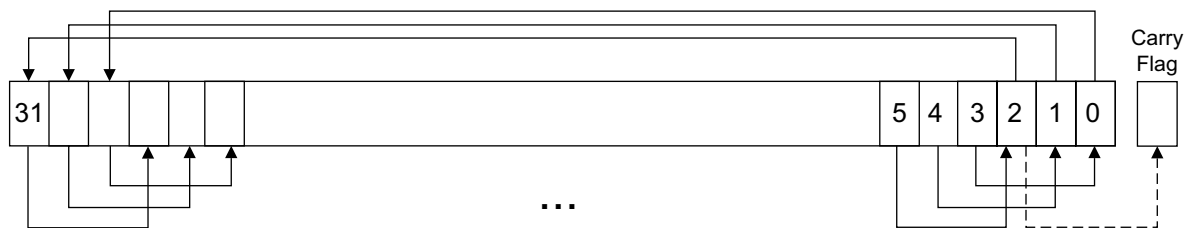
Fig 105. ROR #3
