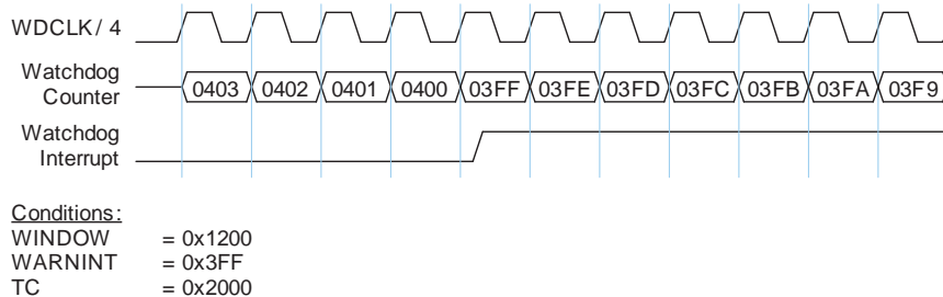
Fig 87. Watchdog Warning Interrupt
