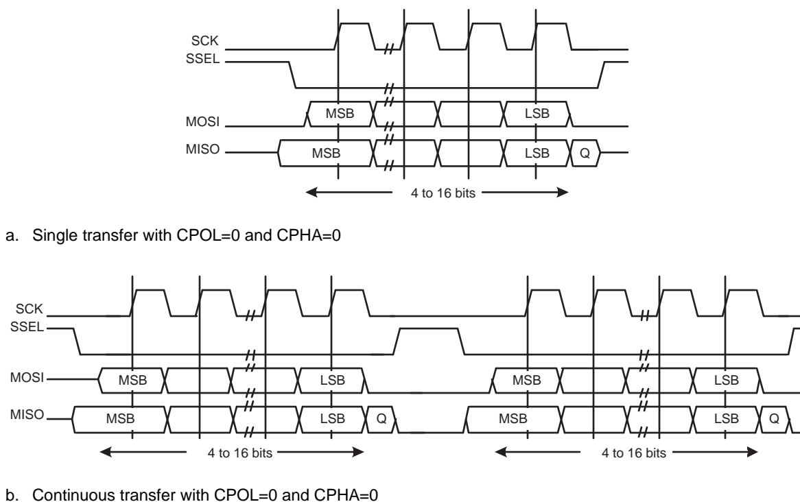
Fig 37. SPI frame format with CPOL=0 and CPHA=0 (a) Single and b) Continuous Transfer)
