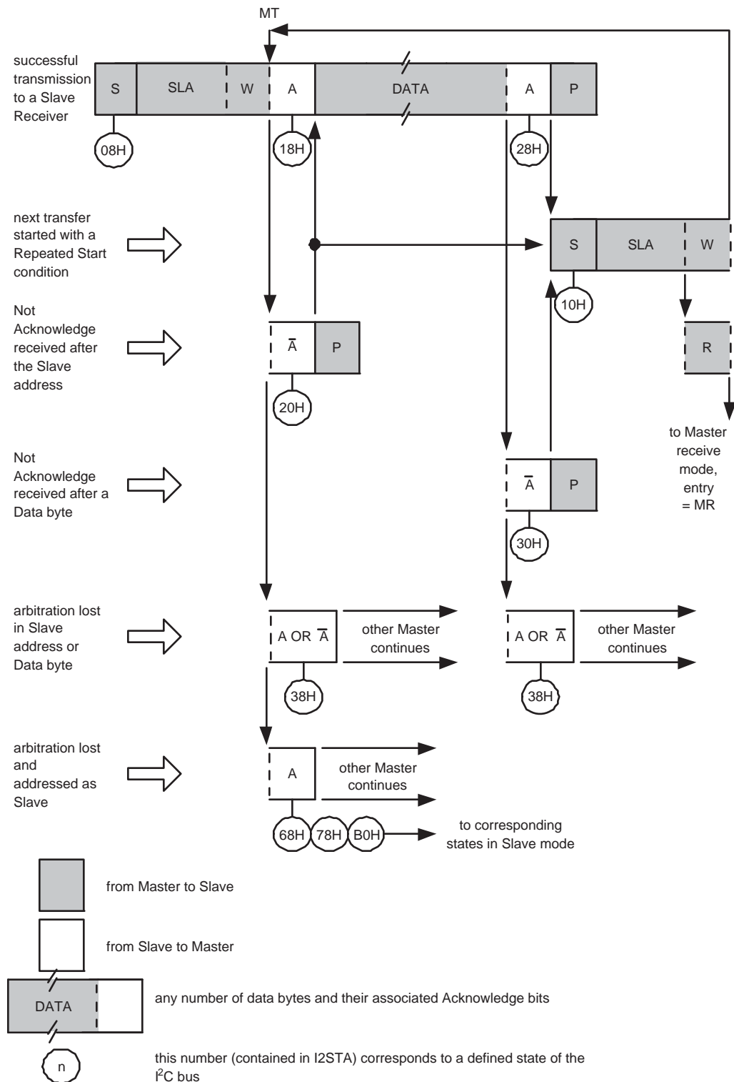
Fig 53. Format and states in the Master Transmitter mode
