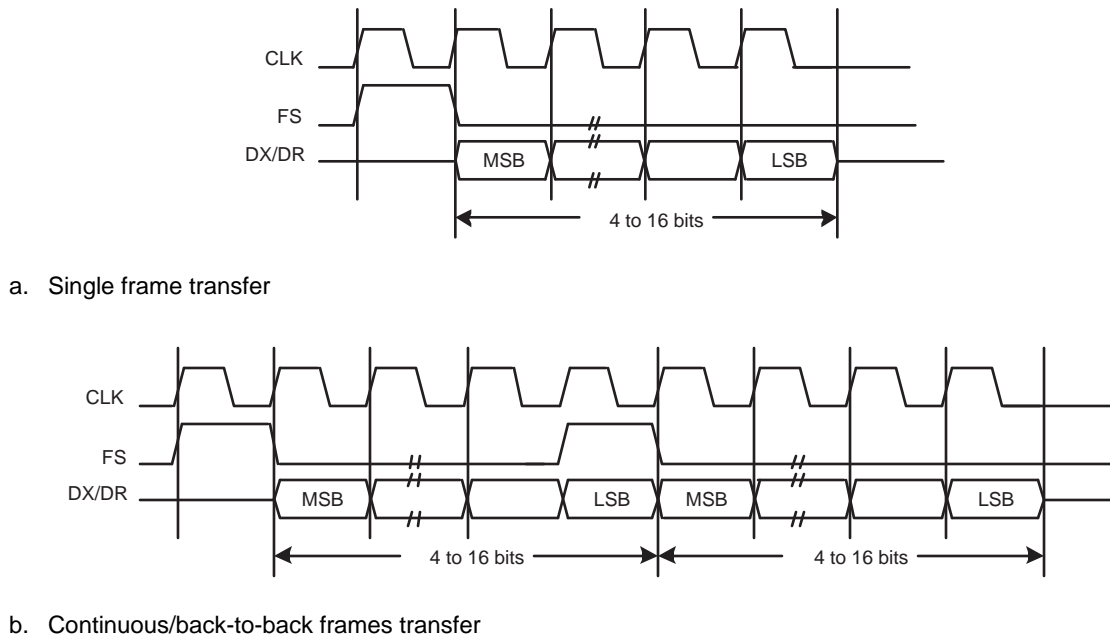
Fig 36. Texas Instruments Synchronous Serial Frame Format: a) Single and b) Continuous/back-to-back Two Frames Transfer
