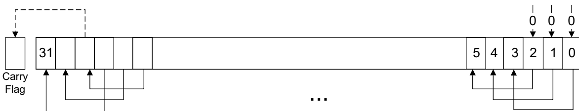
Fig 104. LSL #3
