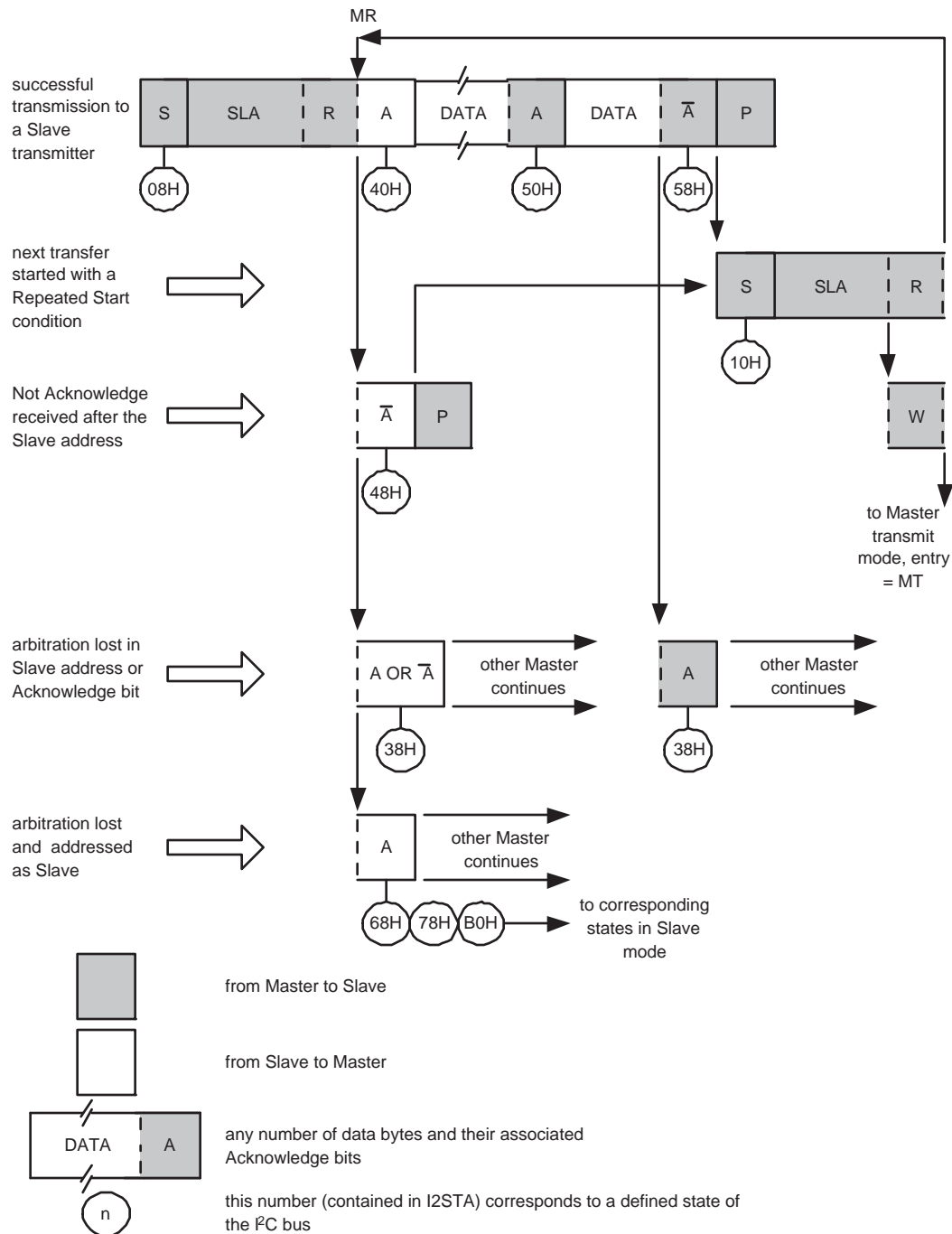
Fig 54. Format and states in the Master Receiver mode
