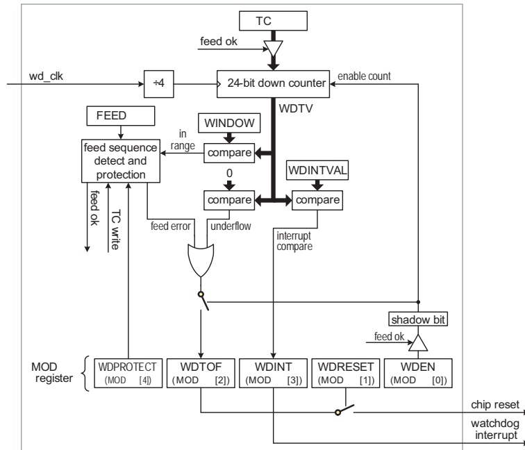
Fig 84. Windowed Watchdog Timer (WWDt) block diagram
