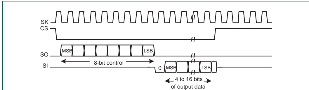
Fig 41. Microwire frame format (single transfer)
