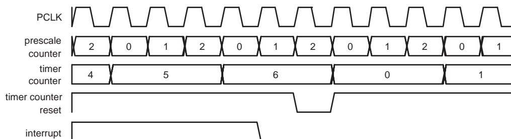
Fig 80. A timer cycle in which PR=2, MRx=6, and both interrupt and reset on match are enabled
