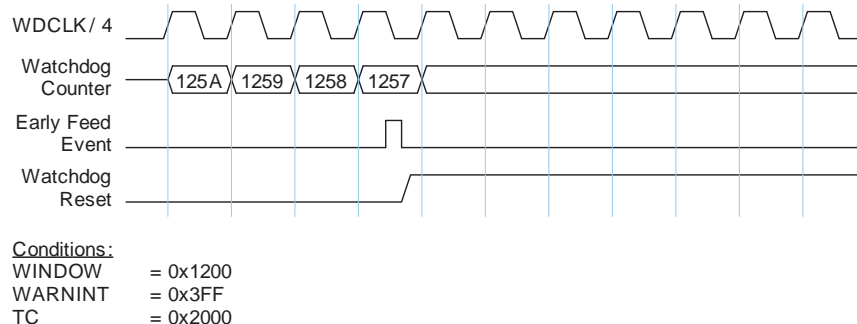
Fig 85. Early Watchdog Feed with Windowed Mode Enabled
