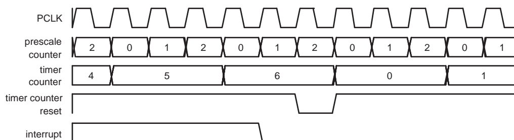
Fig 73. A timer cycle in which PR=2, MRx=6, and both interrupt and reset on match are enabled
