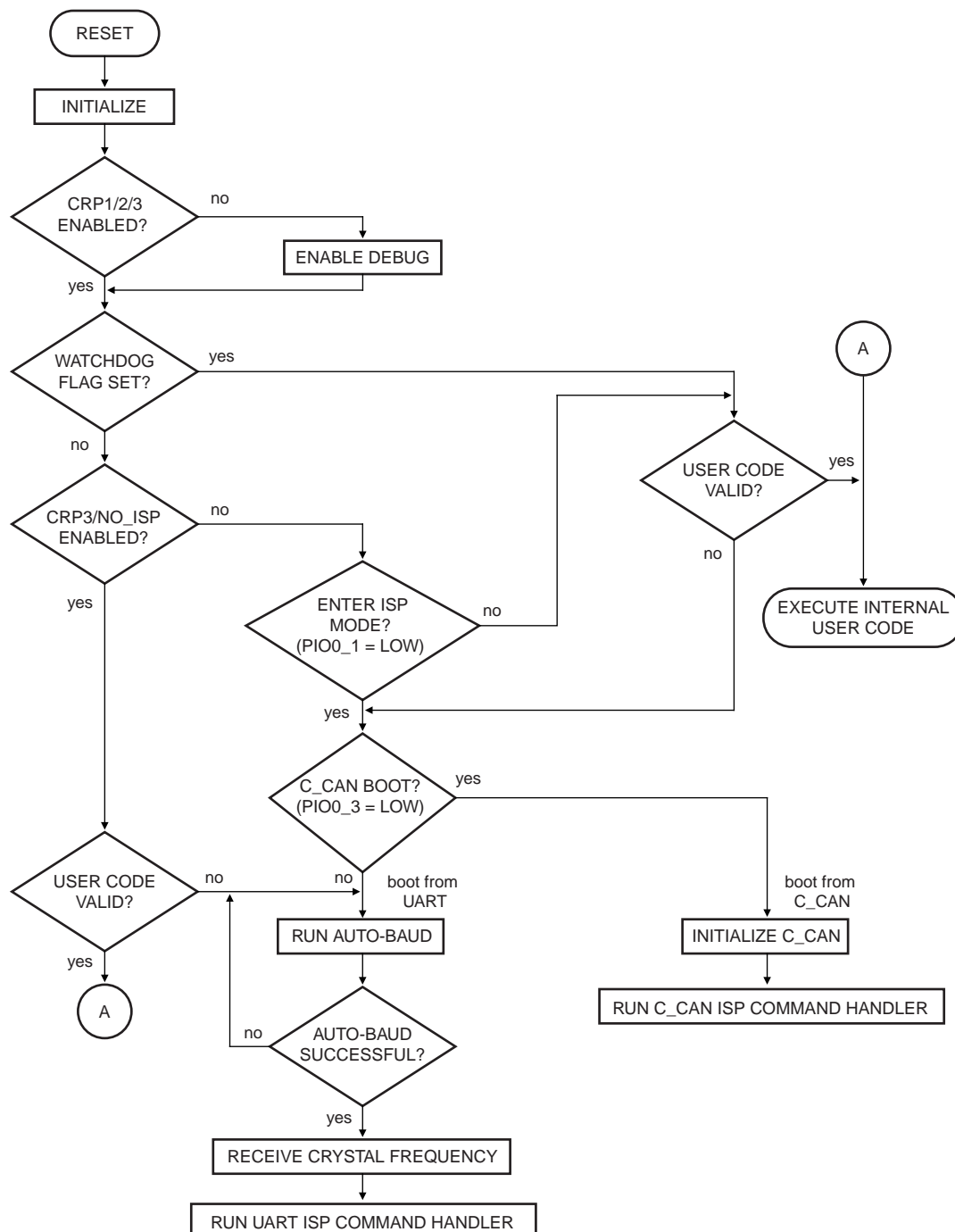
Fig 90. Boot process flowchart
