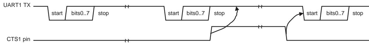
Fig 32. Auto-CTS Functional Timing
