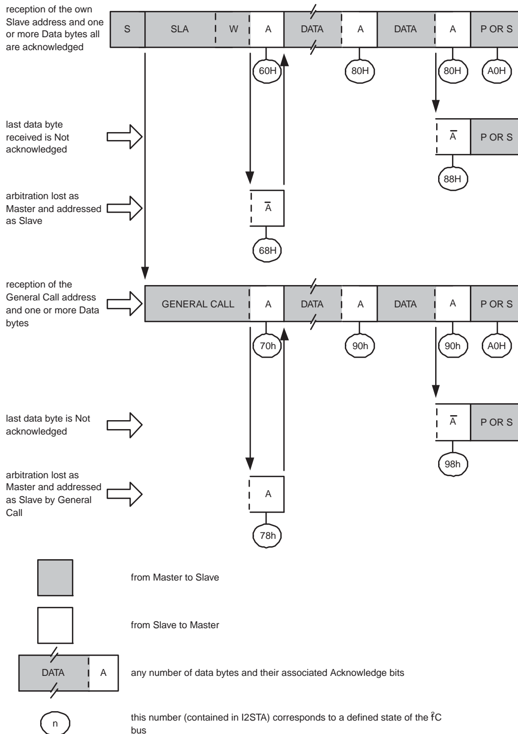
Fig 55. Format and states in the Slave Receiver mode
