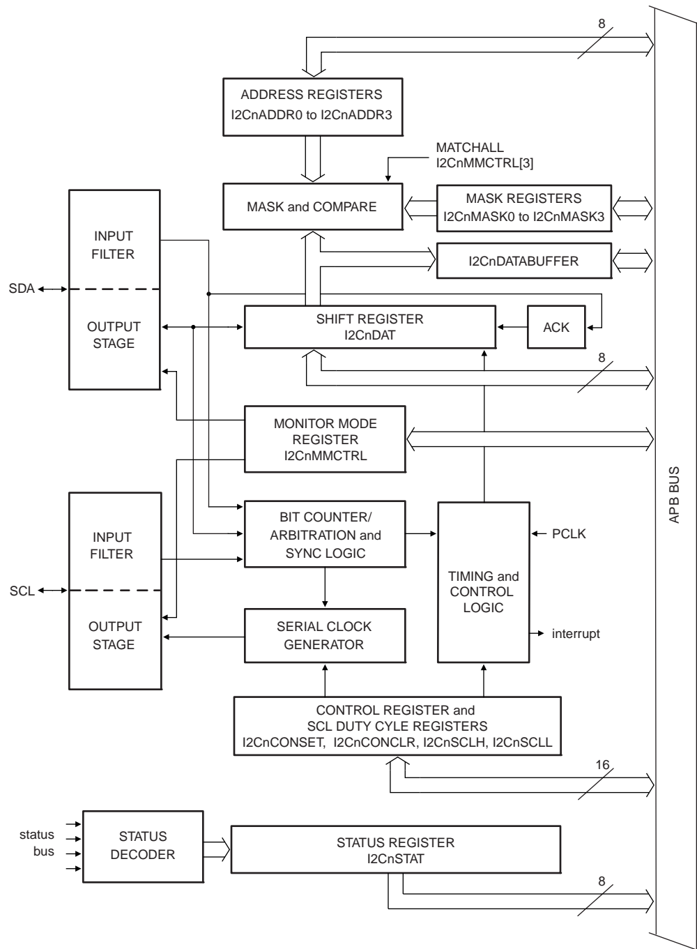
Fig 50. I 2 C serial interface block diagram
