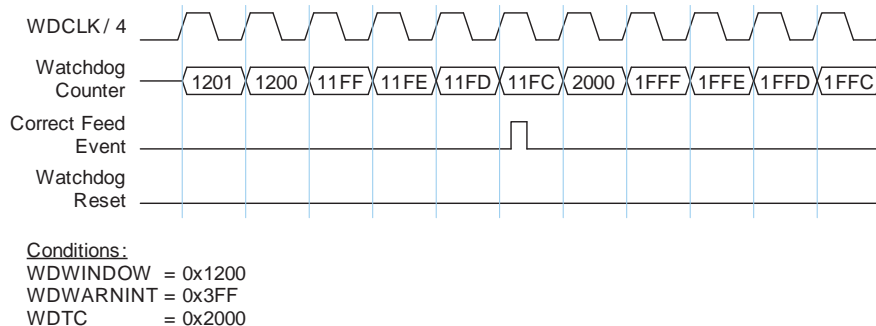
Fig 86. Correct Watchdog Feed with Windowed Mode Enabled
