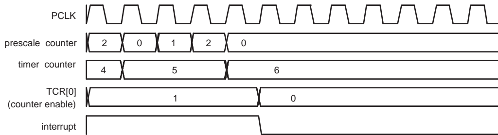
Fig 81. A timer cycle in which PR=2, MRx=6, and both interrupt and stop on match are enabled
