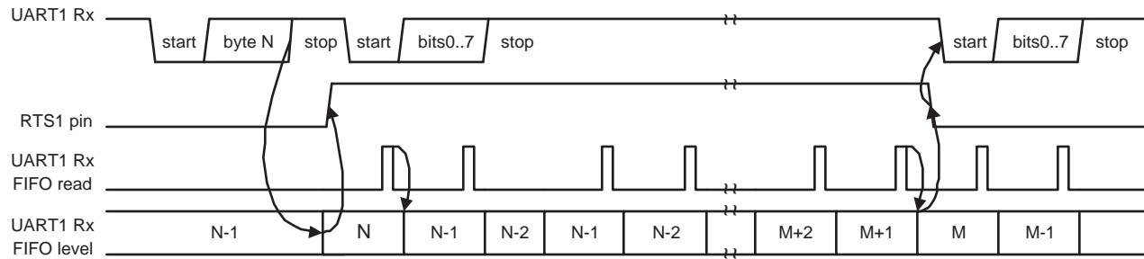
Fig 31. Auto-RTS Functional Timing
