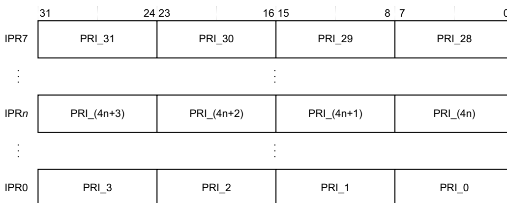
Fig 106. IPR register
