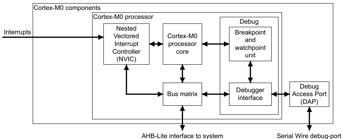
Fig 94. Cortex-M0 implementation
