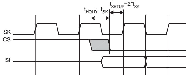
Fig 43. Microwire frame format setup and hold details
