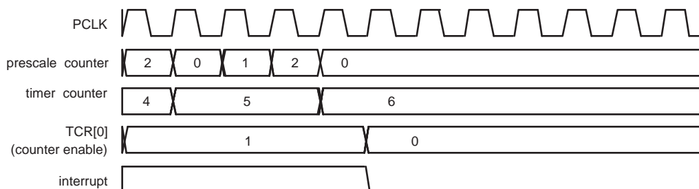
Fig 74. A timer cycle in which PR=2, MRx=6, and both interrupt and stop on match are enabled
