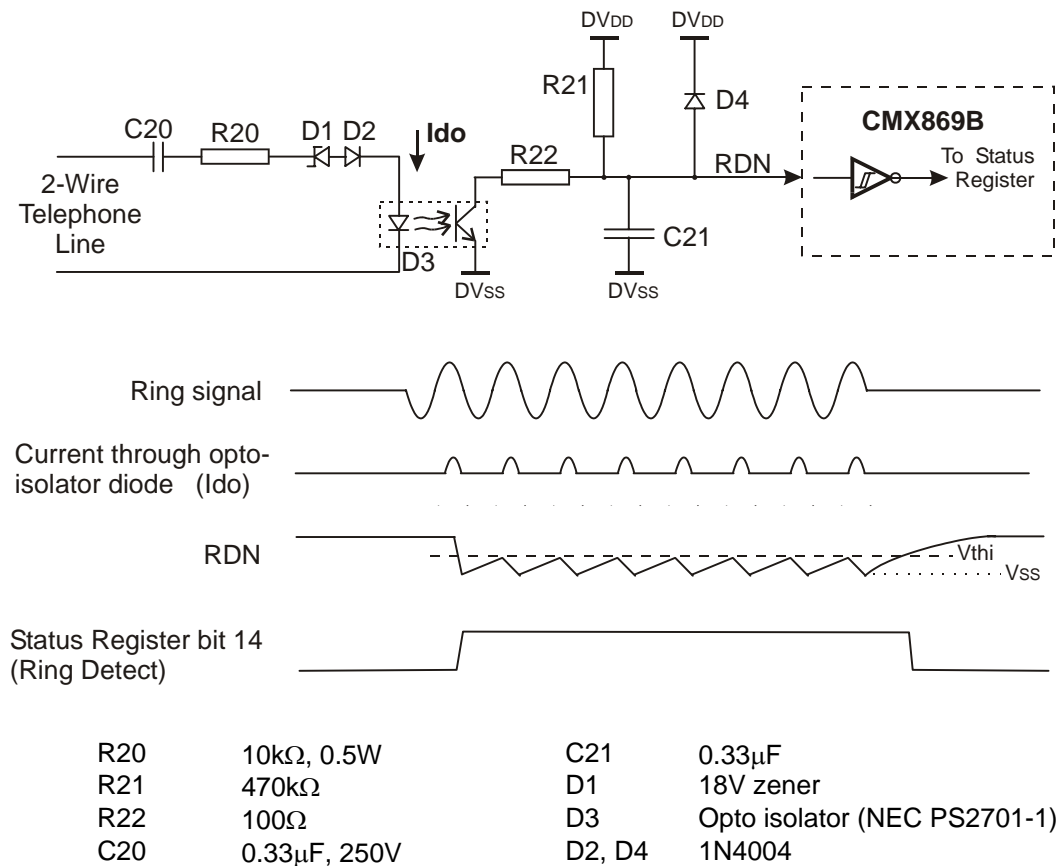
Figure 3 Ring Signal Detector Interface Circuit
