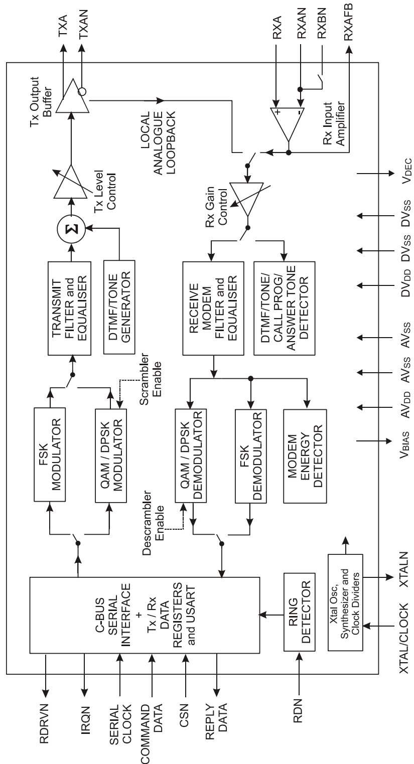
Figure 1 Block Diagram
