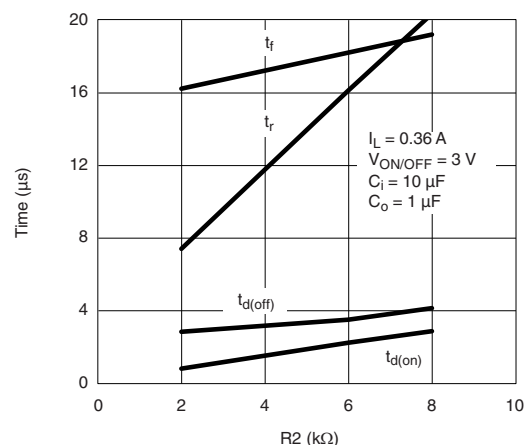
Switching Variation R2 at V_{IN} = 1.8 \text{ V} , R1 = 20 \text{ kΩ}
