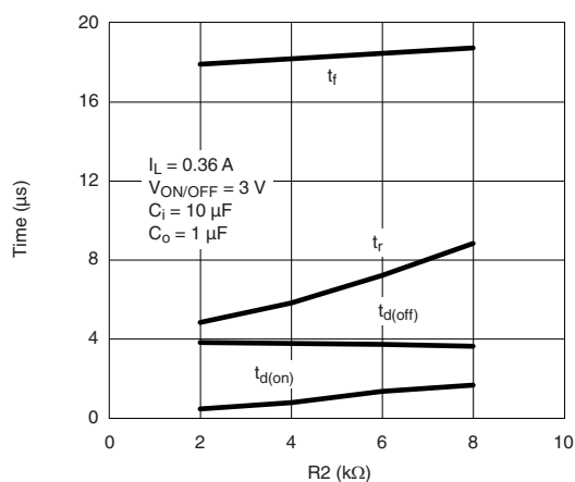
Switching Variation R2 at V_{IN} = 2.5 \text{ V} , R1 = 20 \text{ kΩ}
