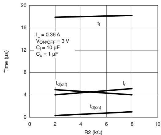
Switching Variation R2 at V_{IN} = 4.5 \text{ V} , R1 = 20 \text{ kΩ}
