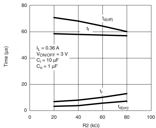
Switching Variation R2 at V_{IN} = 4.5 \text{ V} , R1 = 300 \text{ kΩ}
