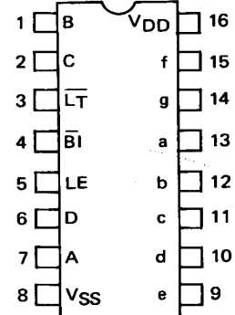
CONNECTION DIAGRAM DIP (TOP VIEW)
