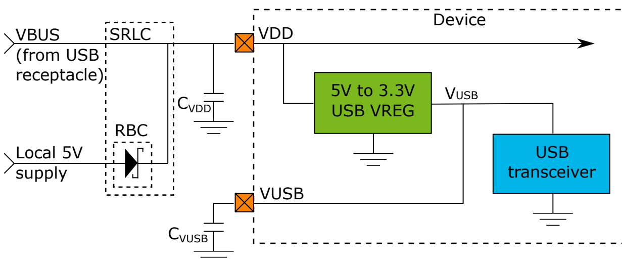
Figure 6-4. Power Configuration 5b5s
