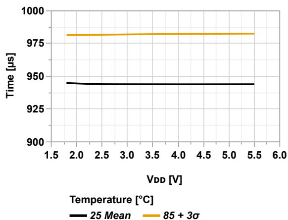
Figure 36-43. Wake-up Time from Power-Down vs. V_{DD} (OSC32K, VREGCTRL = AUTO)
