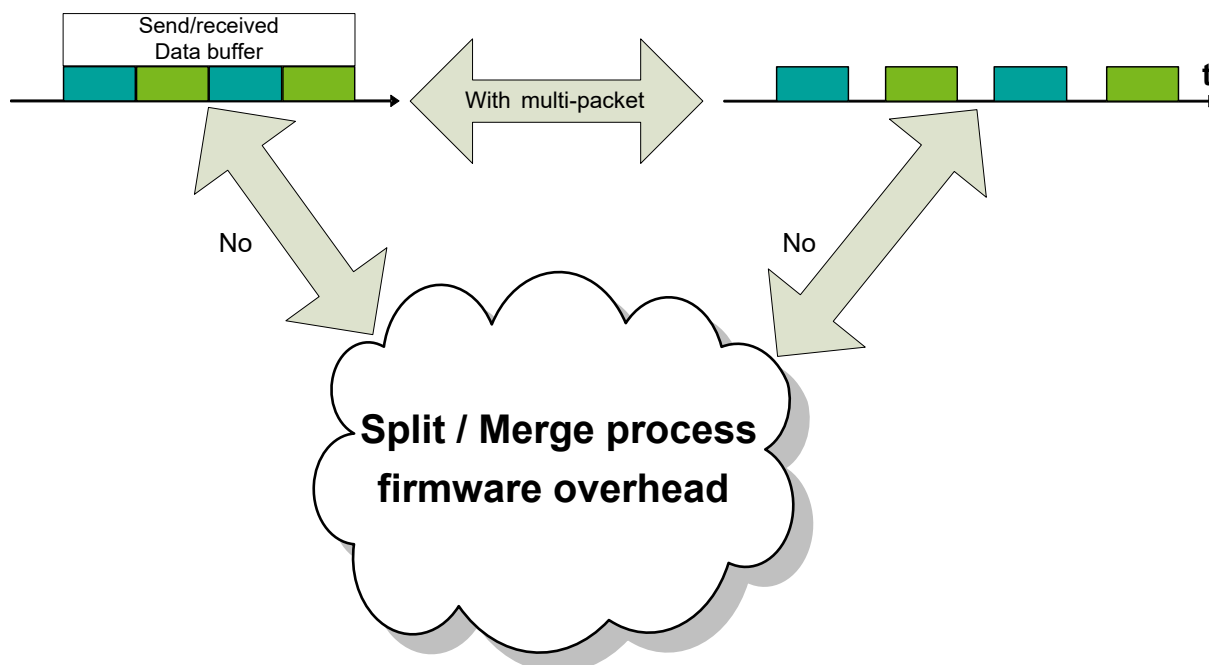
Figure 28-7. Multi-packet Overview
