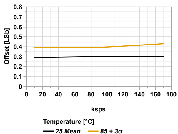
Figure 36-98. Offset Error vs. Sample Rate (ADC Single Ended Mode, V_{\text{REFA}} = V_{\text{DD}} = 3.0\text{V} )
