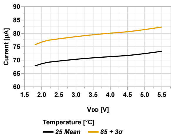
Figure 36-17. AC Power Consumption vs. V_{DD} (CTRLA.POWER = PROFILE0)
