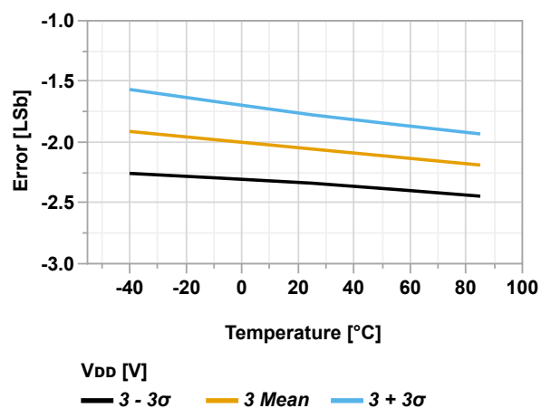
Figure 36-118. Gain Error vs. Temperature ( V_{REFA} = V_{DD} = 3.0V )
