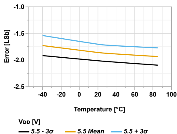
Figure 36-119. Gain Error vs. Temperature ( V_{REFA} = V_{DD} = 5.5V )
