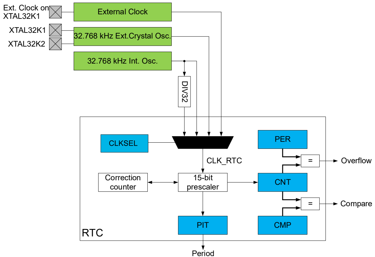
Figure 22-1. Block Diagram
