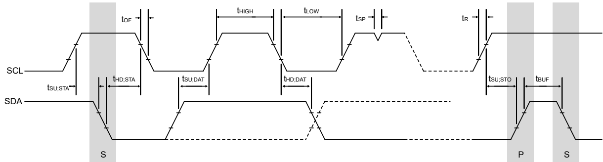
Figure 35-7. TWI - Timing Requirements
