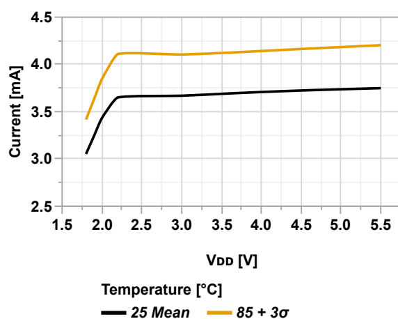
Figure 36-4. Active Power Consumption vs. V_{DD} (MCLKCTRLA.CLKSEL = OSCHF, OSCHF = 24 MHz)
