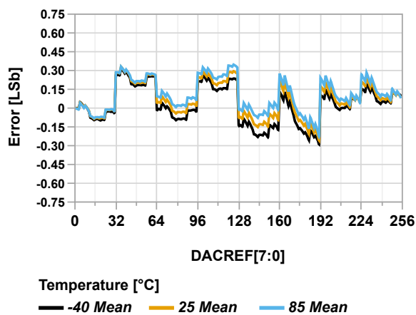
Figure 36-124. INL vs. DAC Code ( V_{\text{REFA}} = V_{\text{DD}} = 3.0\text{V} )
