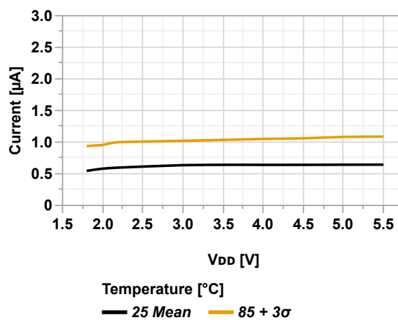
Figure 36-12. Standby Power Consumption vs. V_{DD} (RTC.CLKSEL = OSC32K, HTLLEN = 1)
