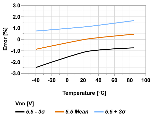
Figure 36-94. ACREF Voltage Error vs. Temperature ( V_{DD} = 5.5V , V_{VREF} = 4.096V )
