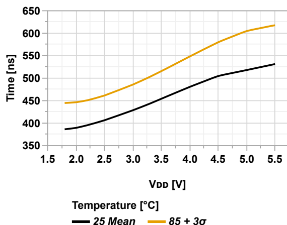
Figure 36-110. Falling Edge Response Time vs. V_{DD} ( V_{CM} = V_{DD}/2 , CTRLA.POWER = 0x02)
