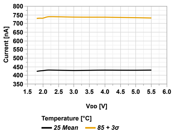
Figure 36-36. WDT Power Consumption vs. V_{DD}
