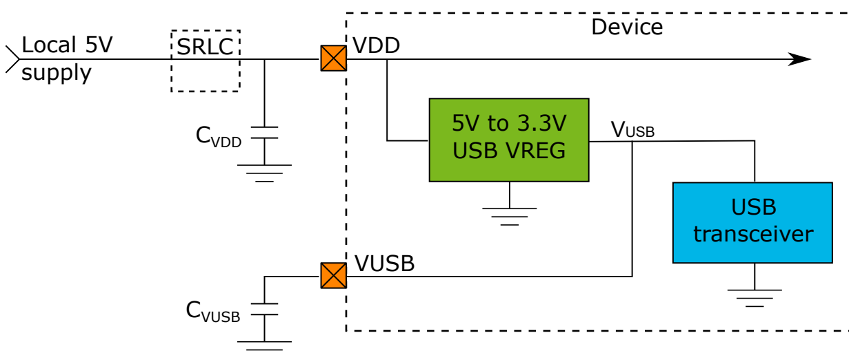
Figure 6-2. Power Configuration 5s
