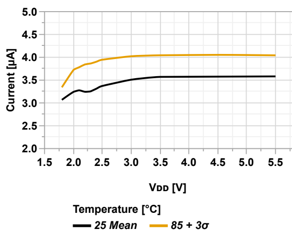
Figure 36-29. TCB Power Consumption vs. V_{DD}
