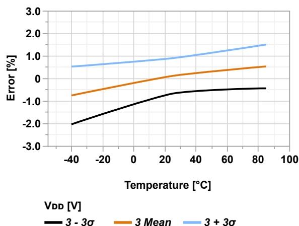
Figure 36-91. ACREF Voltage Error vs. Temperature ( V_{DD} = 3.0V , V_{VREF} = 2.048V )
