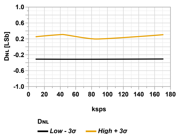
Figure 36-100. DNL vs. Sample Rate (ADC Single Ended Mode, V_{REFA} = V_{DD} = 3.0V , T = 85^{\circ}C )
