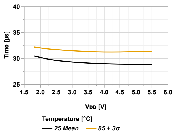
Figure 36-42. Wake-up Time from Power-Down vs. V_{DD} (OSCHF = 4 MHz, VREGCTRL = FULL)
