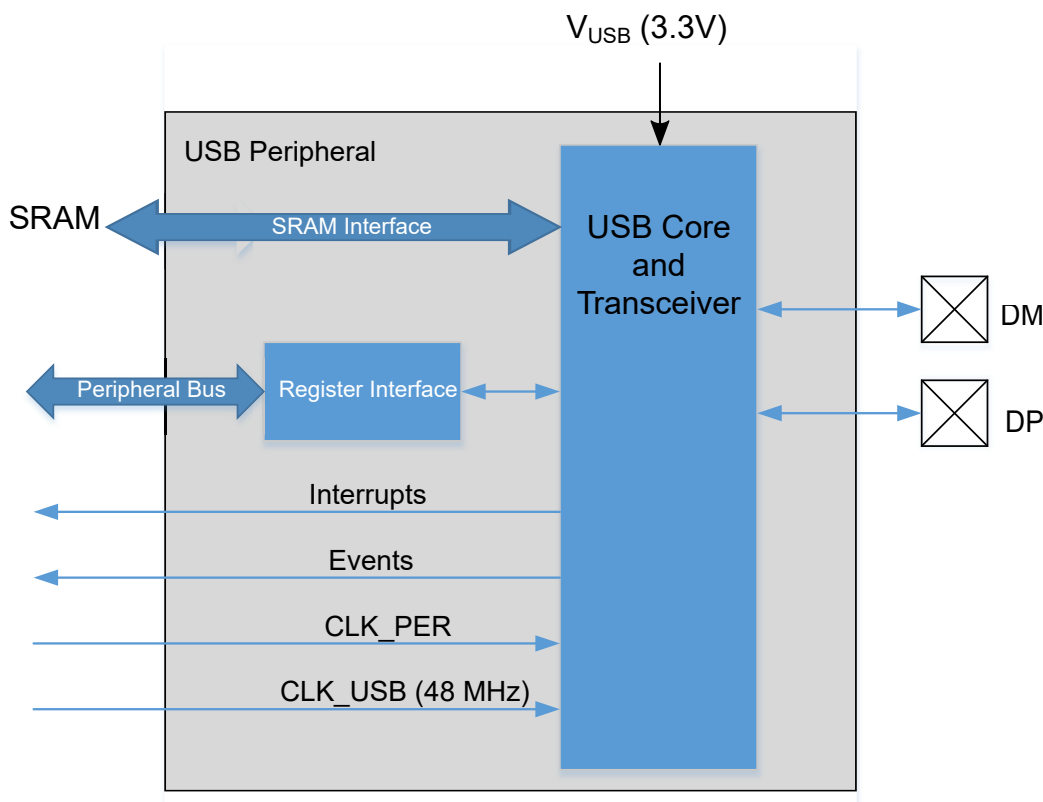
Figure 28-3. USB Block Diagram
