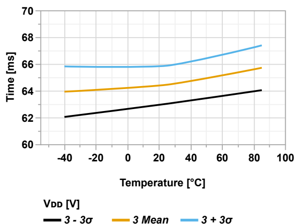
Figure 36-47. Start-up Time vs. Temperature (SYSCFG1 = 0x07, V_{DD} = 3.0V )
