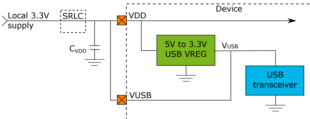
Figure 6-3. Power Configuration 3s
