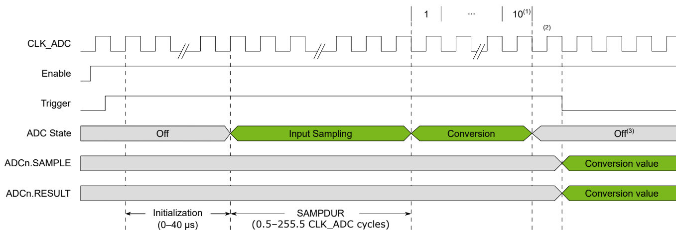
Figure 32-3. Timing Diagram - Single Conversion
