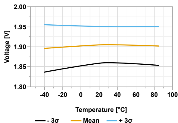
Figure 36-53. BOD Threshold Level vs. Temperature (BODCFG.LVL = 0x02)
