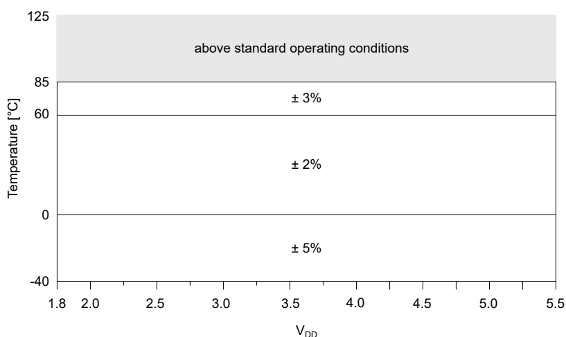
Figure 35-2. Precision Calibrated OSCHF (f OSCHF ≥ 4 MHz) Frequency Accuracy Over Device V DD and Temperature (1)
