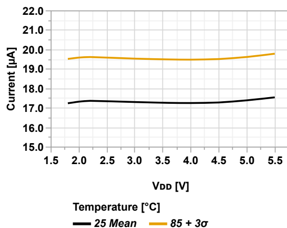
Figure 36-18. AC Power Consumption vs. V_{DD} (CTRLA.POWER = PROFILE1)
