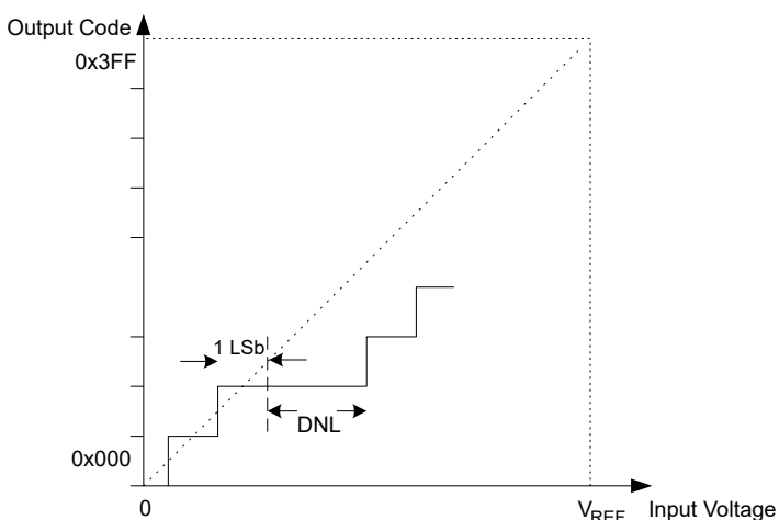
Figure 4-4. Differential Nonlinearity
