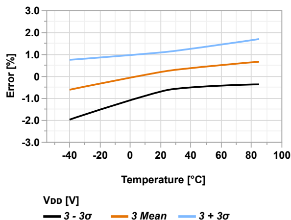
Figure 36-93. ACREF Voltage Error vs. Temperature ( V_{DD} = 3.0V , V_{VREF} = 2.5V )
