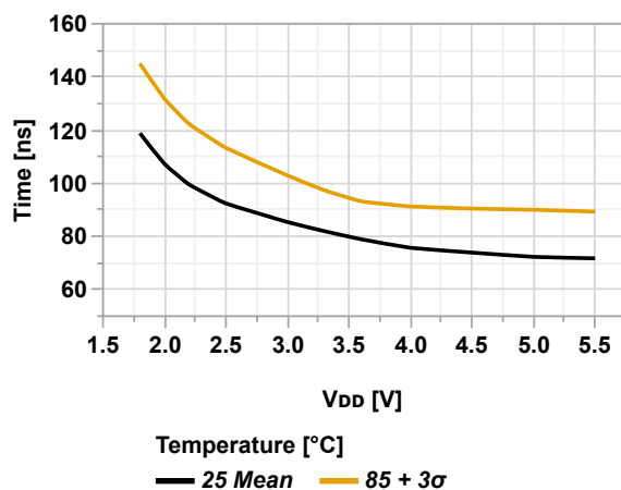
Figure 36-106. Falling Edge Response Time vs. V_{DD} ( V_{CM} = V_{DD}/2 , CTRLA.POWER = 0x00)
