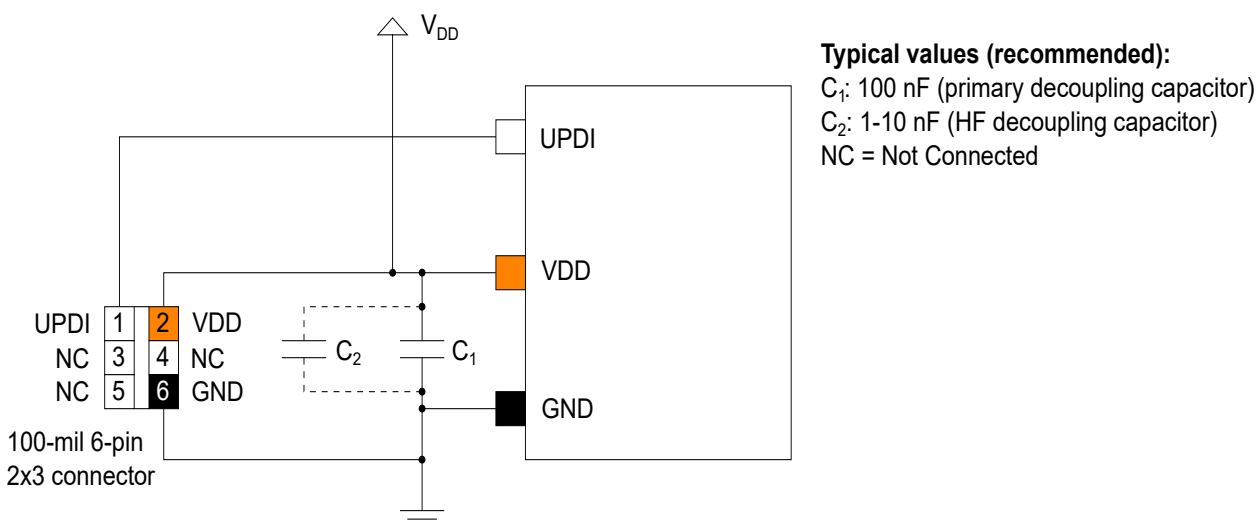
Figure 5-3. Recommended UPDI Programming Circuit Schematic
