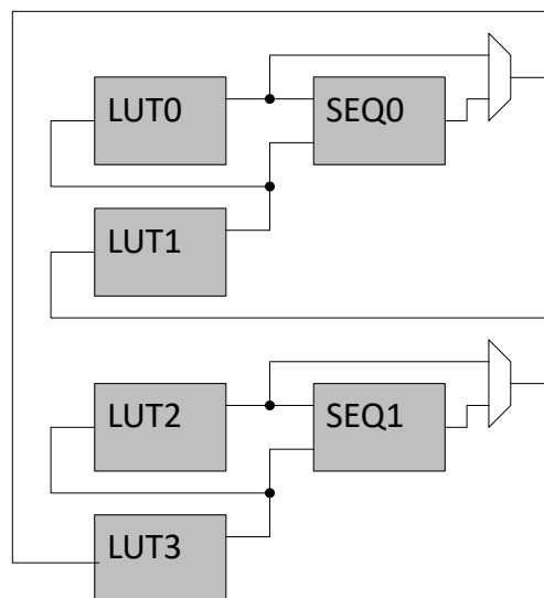
Figure 30-4. Linked LUT Input Selection
