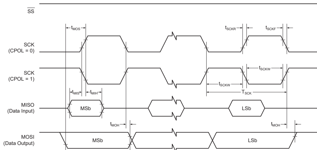
Figure 35-5. SPI - Timing Requirements in Host Mode
