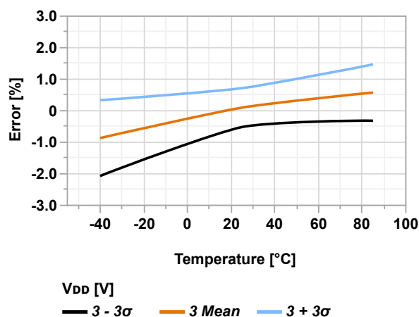
Figure 36-84. ADCOREF Voltage Error vs. Temperature ( V_{DD} = 3.0V , V_{VREF} = 2.048V )
