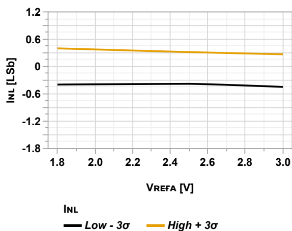
Figure 36-104. INL vs. V_{REFA} (ADC Single Ended Mode @170 kps, V_{DD} = 3.0V , T = 85^{\circ}C )
