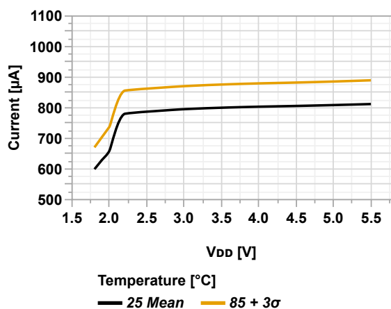
Figure 36-1. Active Power Consumption vs. V_{DD} (MCLKCTRLA.CLKSEL = EXTCLK, EXTCLK = 4 MHz)
