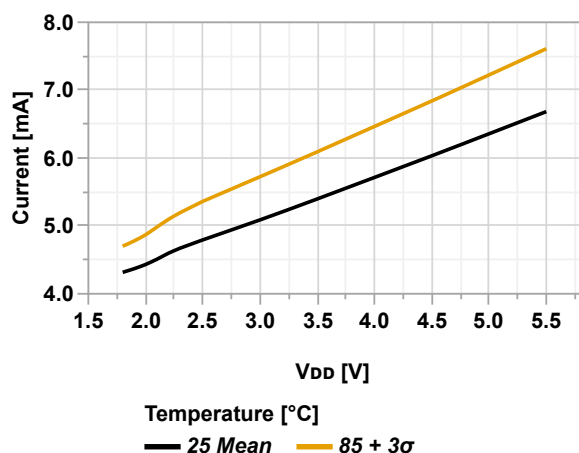
Figure 36-25. Flash Erase Power Consumption vs. V_{DD}
