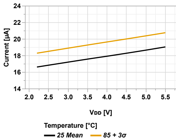
Figure 36-24. BOD Power Consumption vs. V_{DD} (BOD Sampling Mode @32 Hz)
