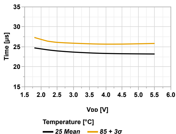
Figure 36-40. Wake-up Time from Power-Down vs. V_{DD} (OSCHF = 16 MHz, VREGCTRL = FULL)
