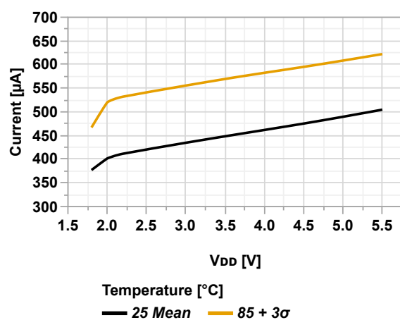
Figure 36-21. ADC Power Consumption vs. V_{DD} (ADC @170 kps)
