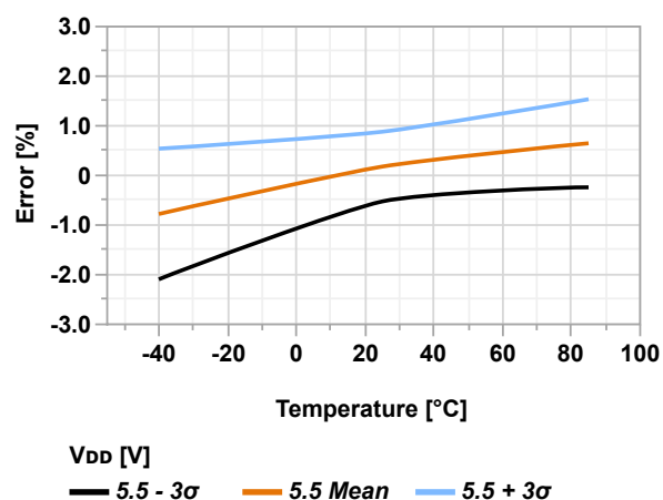
Figure 36-87. ADC0REF Voltage Error vs. Temperature ( V_{DD} = 5.5V , V_{VREF} = 4.096V )
