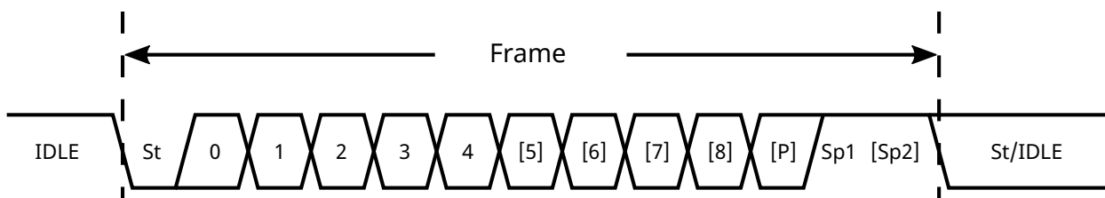
Figure 25-2. Frame Formats
