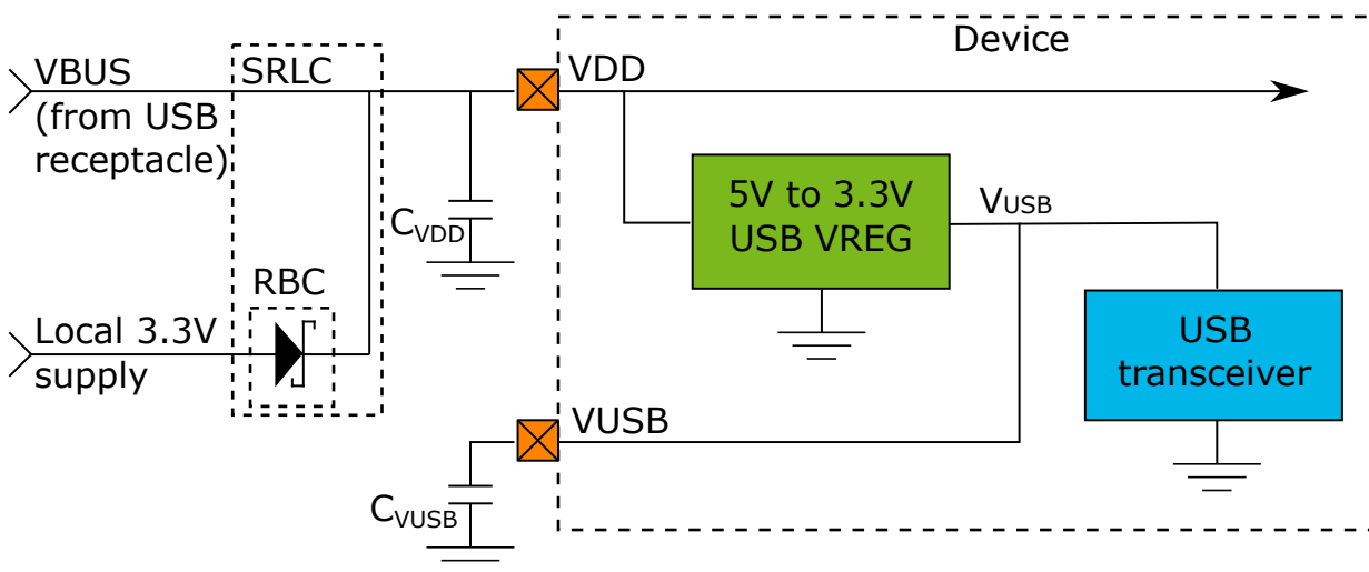
Figure 6-5. Power Configuration 5b3s
