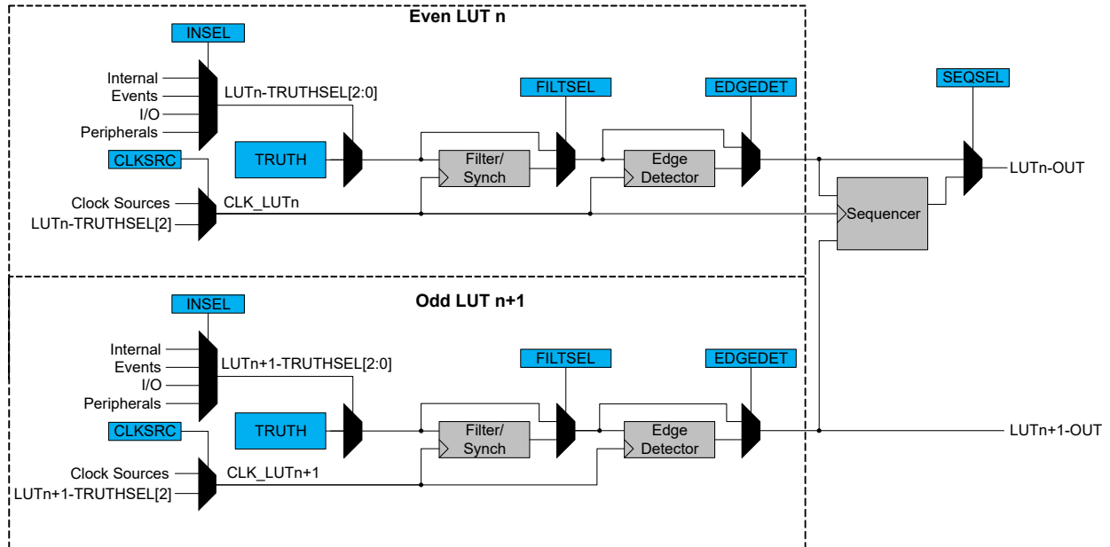
Figure 30-1. CCL Block Diagram
