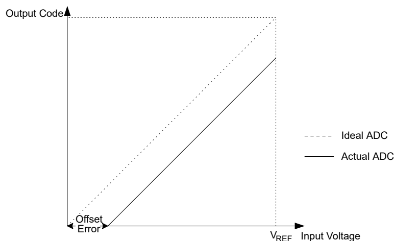
Figure 4-1. Offset Error
