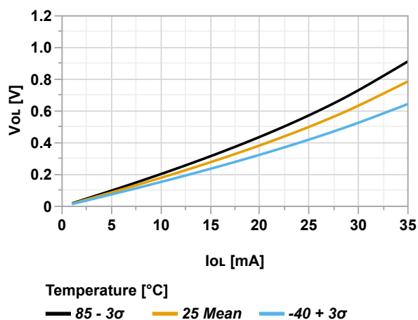
Figure 36-79. Output Pin - Maximum V_{OL} vs. Current, V_{DD} = 5.5V
