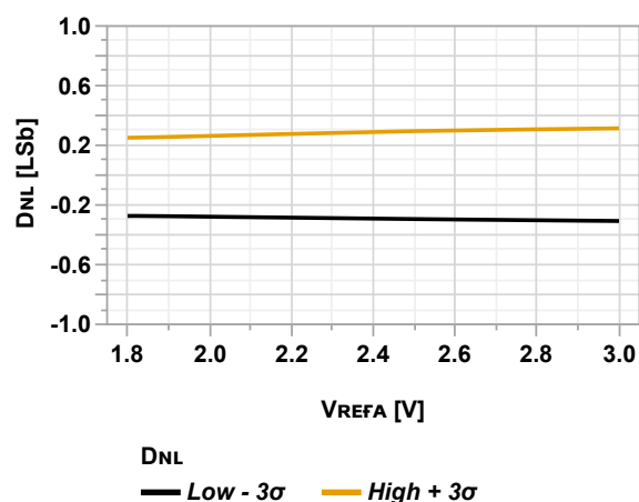
Figure 36-101. DNL vs. V_{REFA} (ADC Single Ended Mode @170 kps, V_{DD} = 3.0V , T = 85^{\circ}C )
