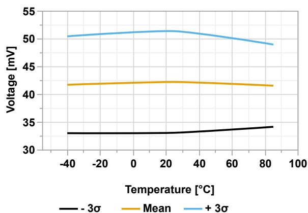
Figure 36-57. BOD Hysteresis vs. Temperature (BODCFG.LVL = 0x02)
