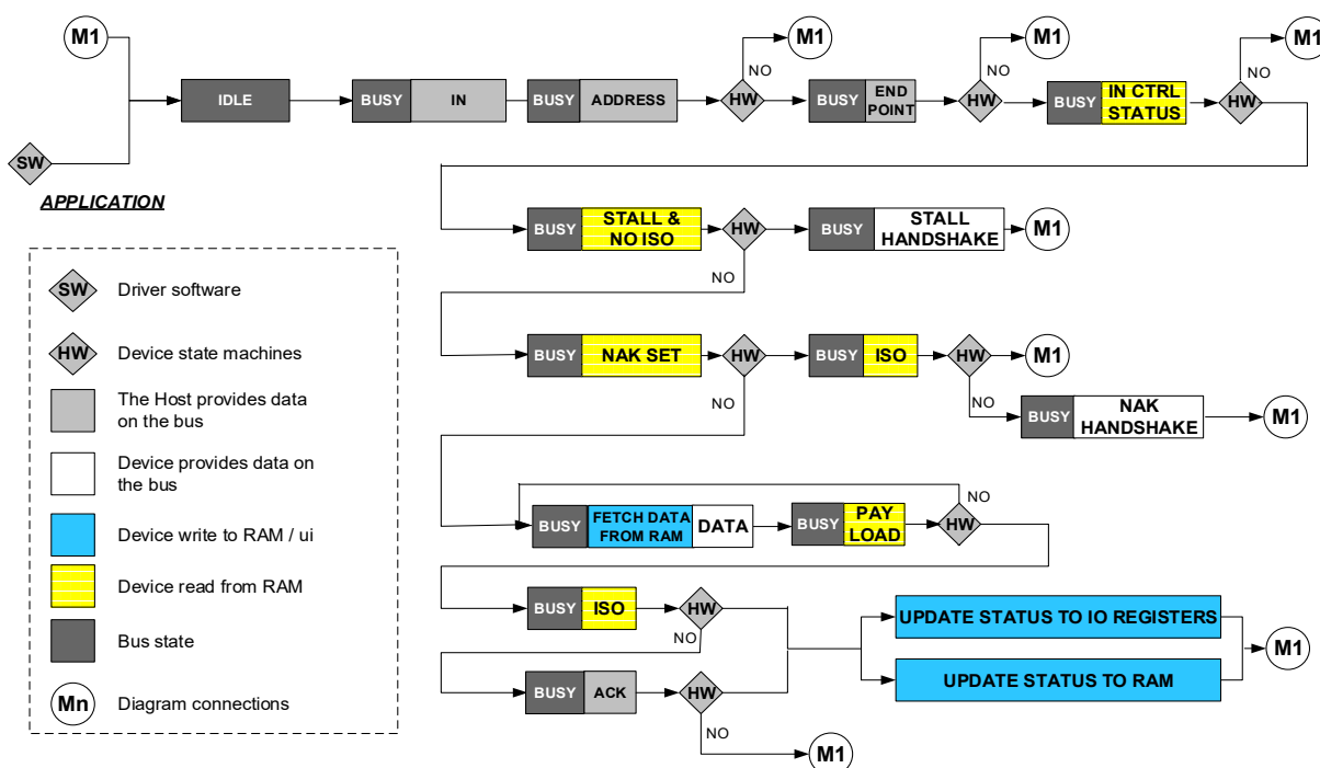
Figure 28-6. IN Transaction
