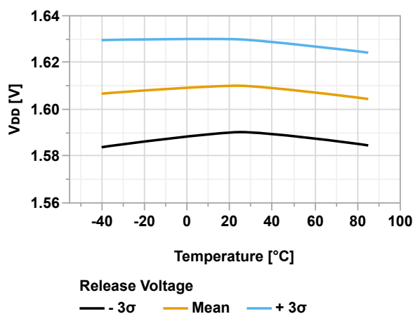
Figure 36-49. \overline{POR} Release Voltage vs. Temperature
