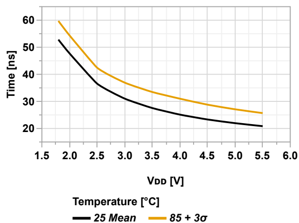
Figure 36-65. Rise Time vs. V_{DD} (PORTCTRL.SRL = 0x01)
