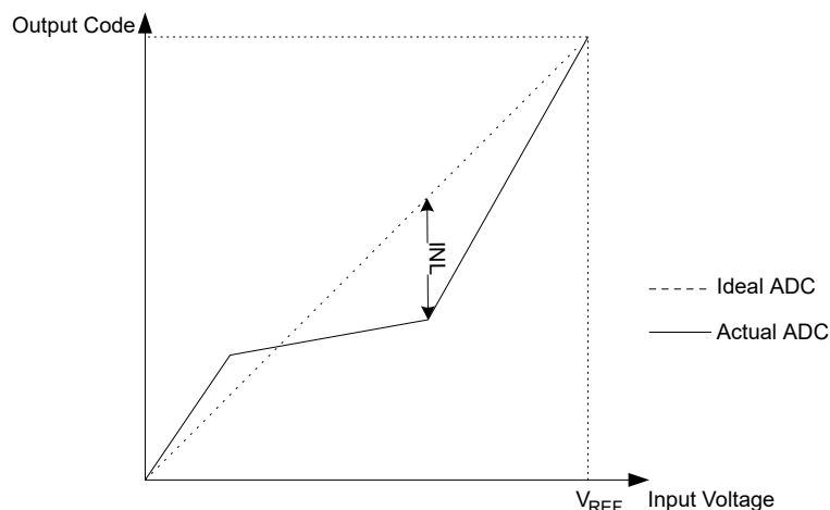
Figure 4-3. Integral Nonlinearity
