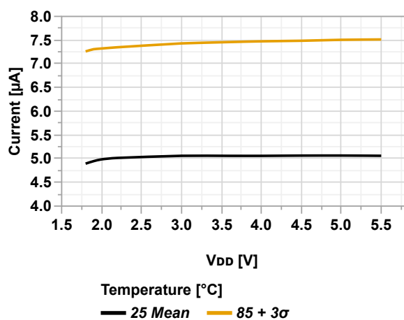
Figure 36-5. Active Power Consumption vs. V_{DD} (MCLKCTRLA.CLKSEL = OSC32K)
