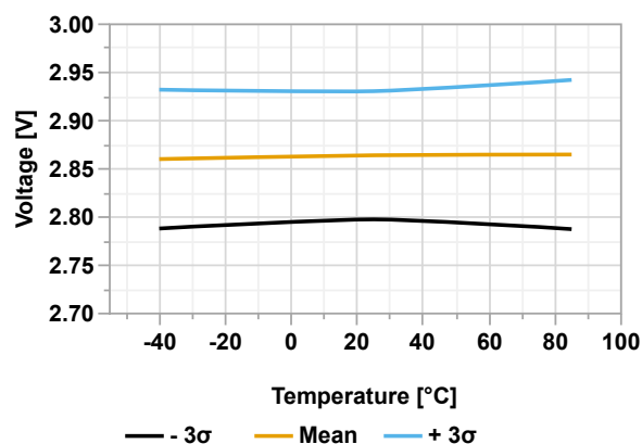
Figure 36-54. BOD Threshold Level vs. Temperature (BODCFG.LVL = 0x03)
