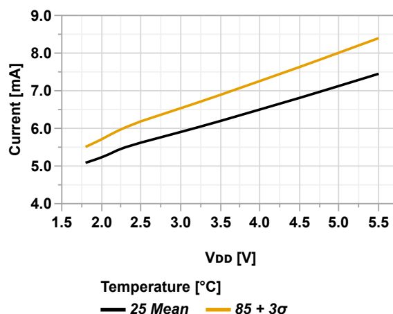
Figure 36-26. Flash Write Power Consumption vs. V_{DD}
