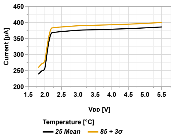
Figure 36-8. Idle Power Consumption vs. V_{DD} (MCLKCTRLA.CLKSEL = OSCHF, OSCHF = 4 MHz)
