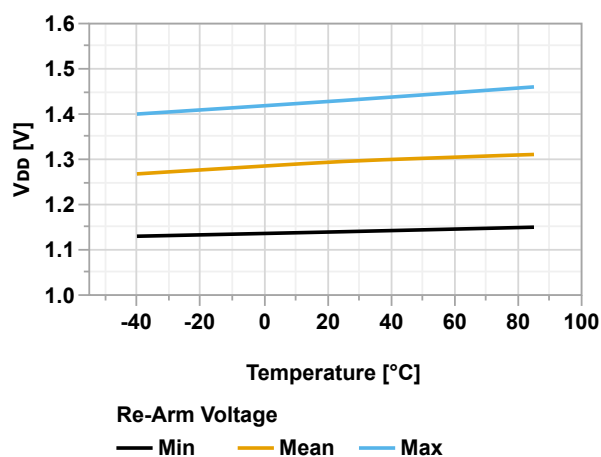
Figure 36-50. \overline{POR} Re-Arm Voltage vs. Temperature
