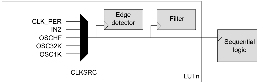
Figure 30-11. Clock Source Settings
