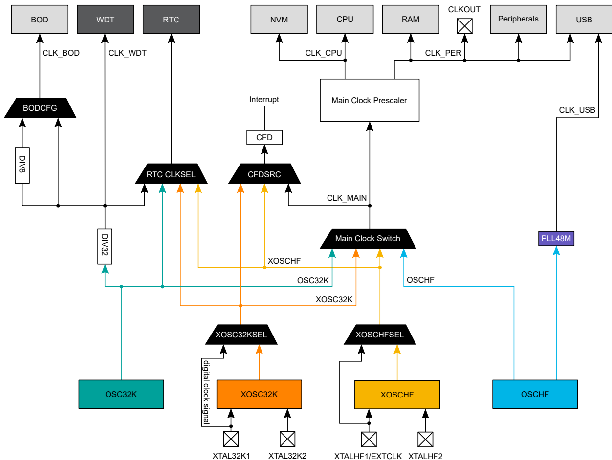
Figure 12-1. CLKCTRL Block Diagram
