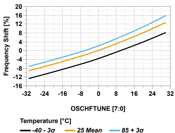
Figure 36-37. Frequency Shift vs. OSCHFTUNE Code ( V_{DD} = 3.0V )
