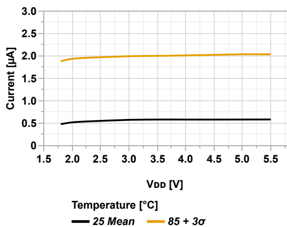
Figure 36-11. Standby Power Consumption vs. V_{DD} (RTC.CLKSEL = OSC32K, HTLLEN = 0)
