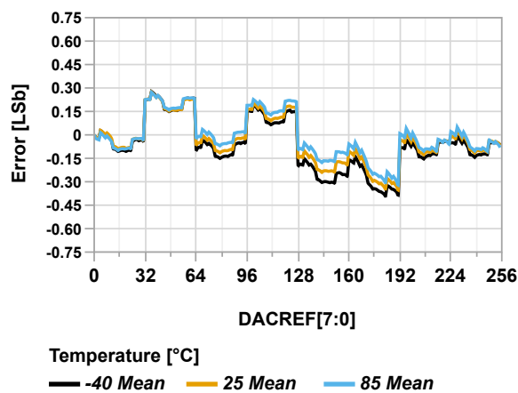
Figure 36-125. INL vs. DAC Code ( V_{\text{REFA}} = V_{\text{DD}} = 5.5\text{V} )
