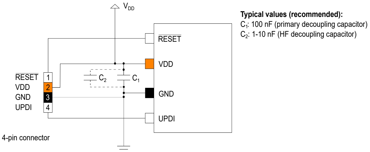
Figure 5-4. Recommended UPDI Programming Circuit Schematic
