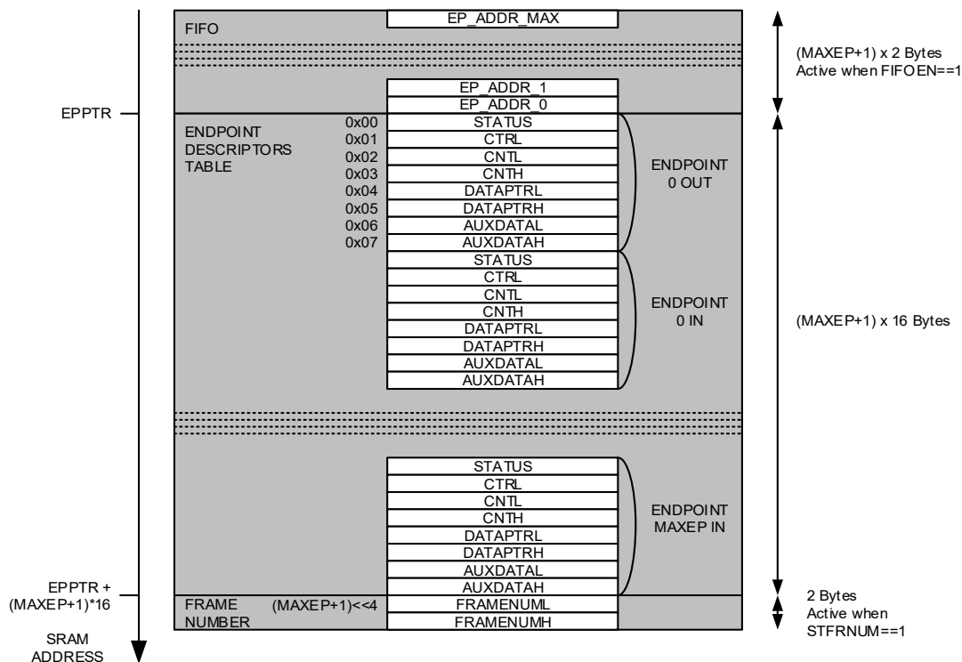
Figure 28-9. USB Memory Mapping (Descriptor table, FIFO, Frame number, Endpoint buffers) In RAM
