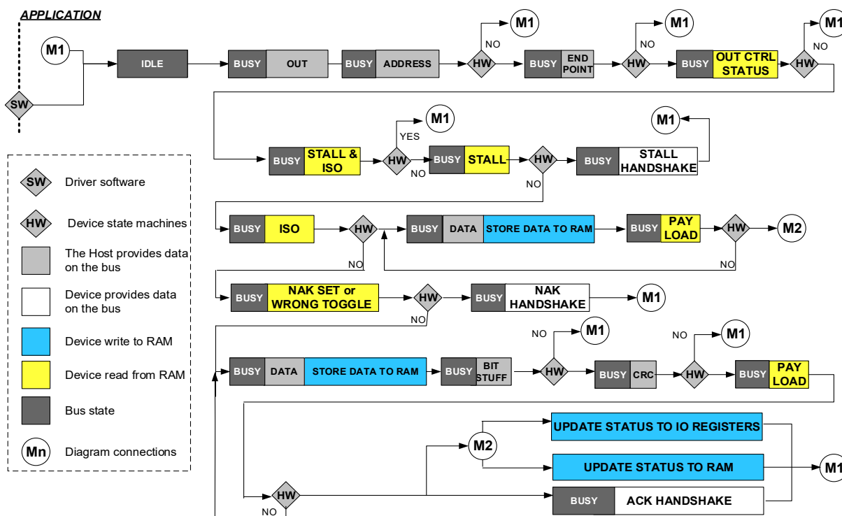
Figure 28-5. OUT Transaction
