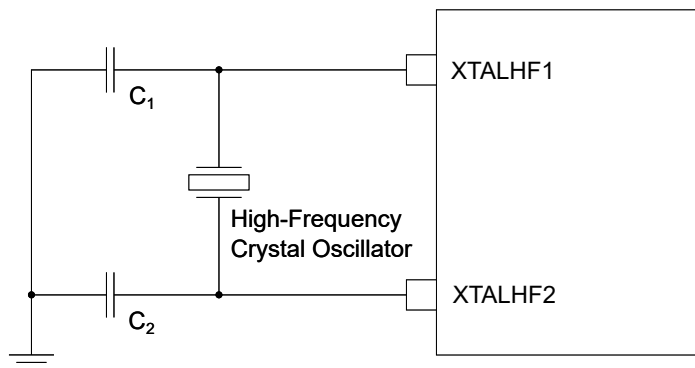
Figure 5-6. Recommended External High-Frequency Oscillator Connection Circuit Schematic
