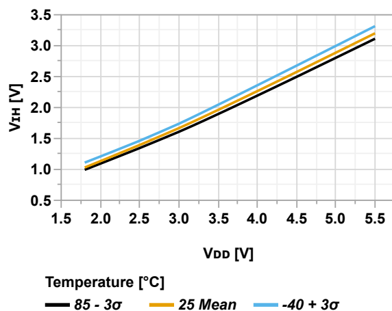
Figure 36-72. Input Pin SMBus - Minimum V_{IH} vs. V_{DD}
