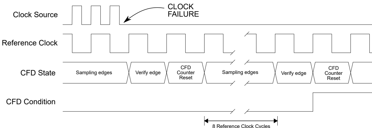
Figure 12-6. Clock Failure Detection (CFD) Timing Diagram
