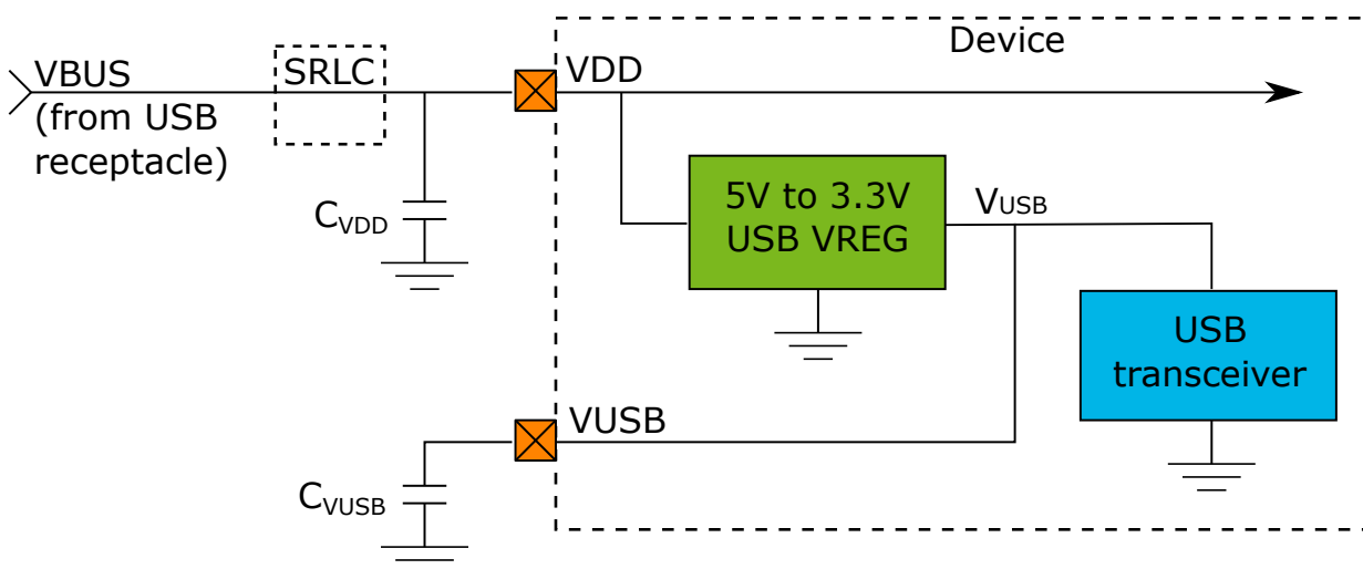
Figure 6-1. Power Configuration 5b
