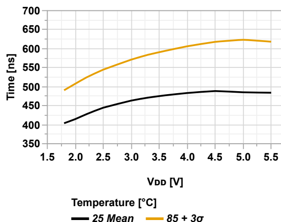
Figure 36-111. Rising Edge Response Time vs. V_{DD} ( V_{CM} = V_{DD}/2 , CTRLA.POWER = 0x02)
