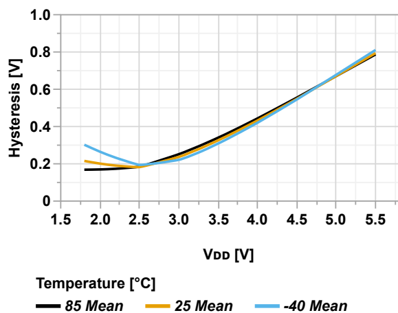
Figure 36-68. Input Pin with Schmitt Trigger - Hysteresis vs. V_{DD}
