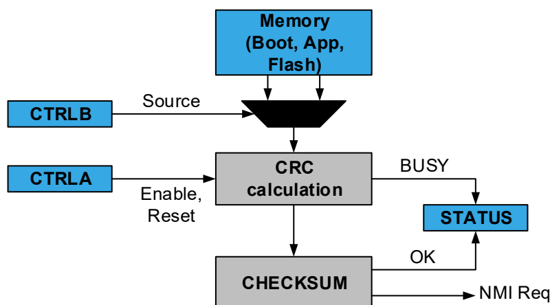
Figure 29-1. Cyclic Redundancy Check Block Diagram
