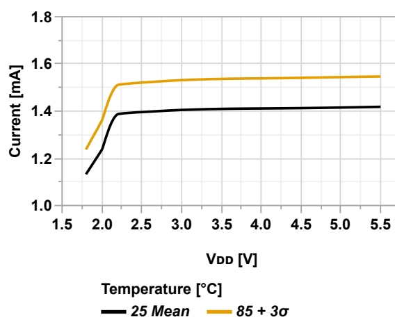
Figure 36-9. Idle Power Consumption vs. V_{DD} (MCLKCTRLA.CLKSEL = OSCHF, OSCHF = 24 MHz)
