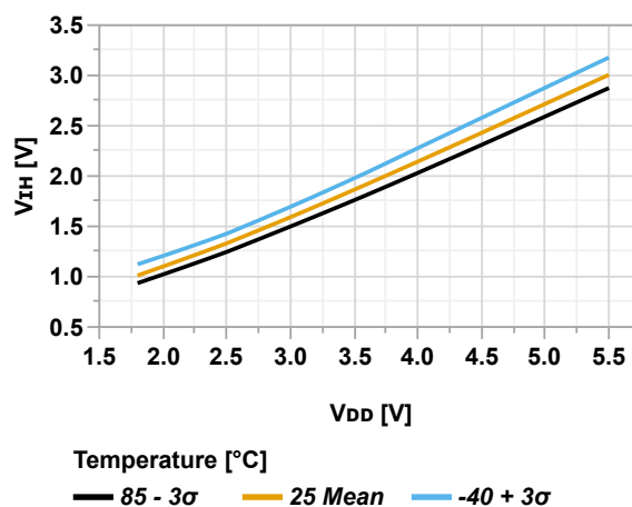
Figure 36-67. Input Pin with Schmitt Trigger - Minimum V_{IH} vs. V_{DD}
