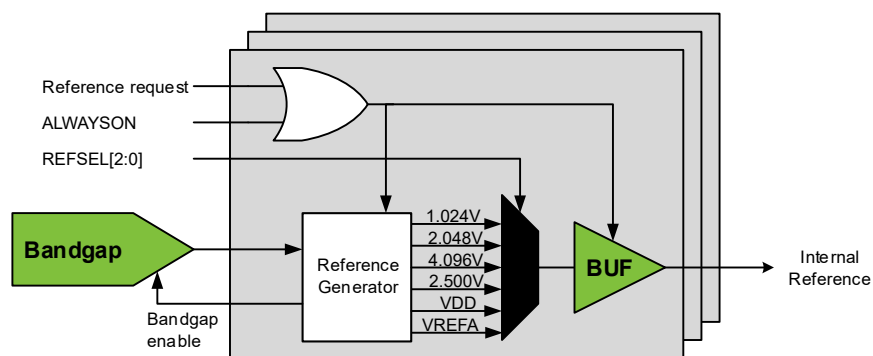
Figure 20-1. VREF Block Diagram
