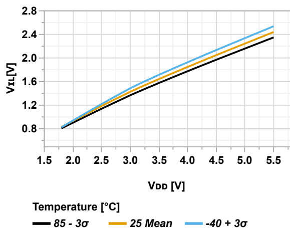
Figure 36-71. Input Pin SMBus - Maximum V_{IL} vs. V_{DD}
