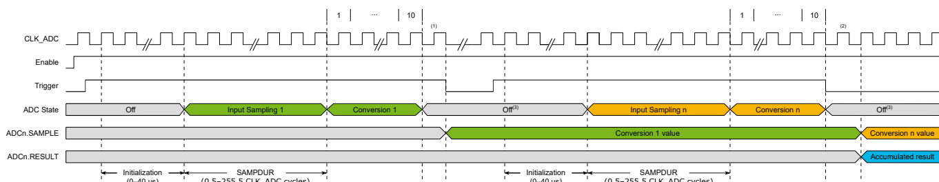
Figure 32-4. Timing Diagram - Series Accumulation
