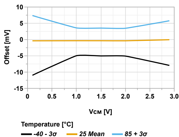
Figure 36-114. Input Offset vs. Common Mode Voltage ( V_{DD} = 3.0V )
