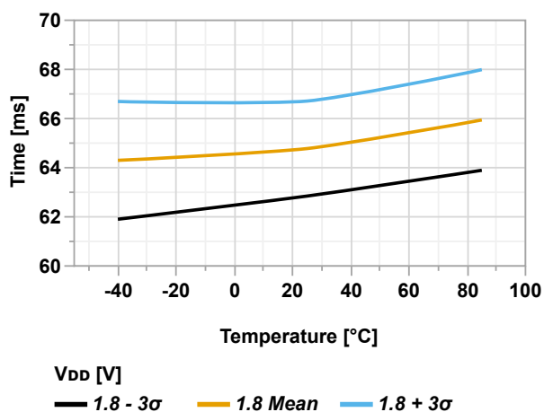
Figure 36-46. Start-up Time vs. Temperature (SYSCFG1 = 0x07, V_{DD} = 1.8V)
