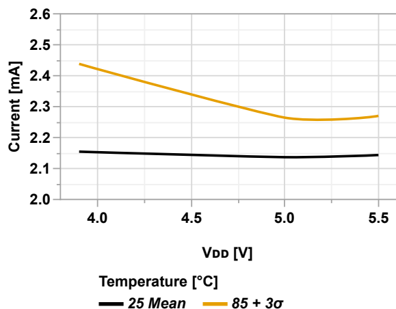
Figure 36-35. USBVREG Power Consumption vs. V_{DD}
