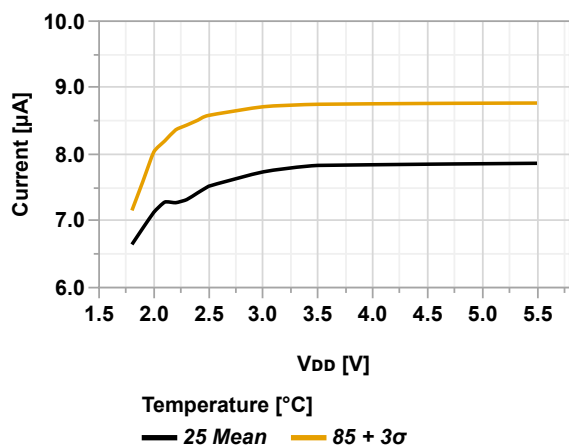
Figure 36-30. TWI Power Consumption vs. V_{DD} (TWI Host Mode @100 kHz)
