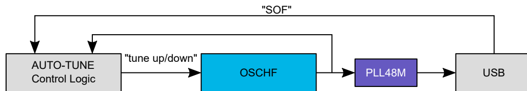
Figure 12-4. OSCHF Start-Of-Frame Auto-Tune Block Diagram
