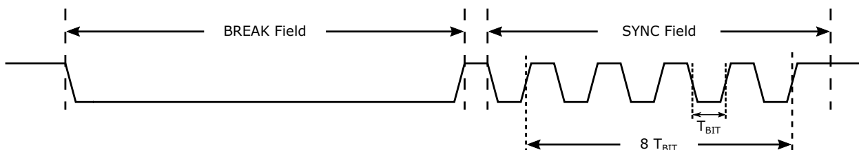
Figure 25-9. Auto-Baud Timing
