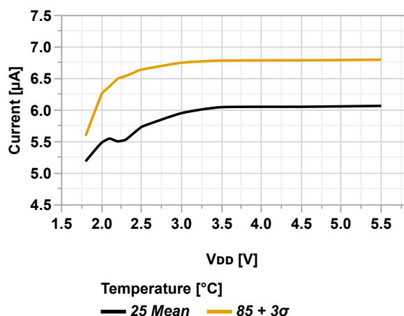
Figure 36-28. TCA Power Consumption vs. V_{DD}
