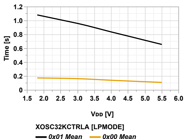
Figure 36-38. Typical XOSC32K Start-up Time vs. V_{DD} ( T = 25^{\circ}\text{C} )
