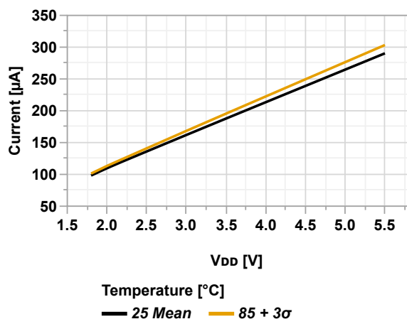
Figure 36-16. Reset Power Consumption vs. V_{DD}
