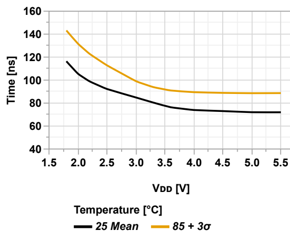
Figure 36-107. Rising Edge Response Time vs. V_{DD} ( V_{CM} = V_{DD}/2 , CTRLA.POWER = 0x00)
