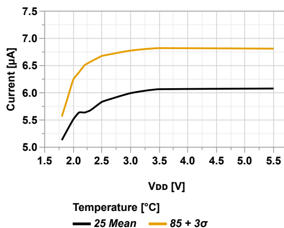
Figure 36-31. TWI Power Consumption vs. V_{DD} (TWI Client Mode @100 kHz)
