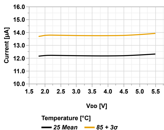
Figure 36-19. AC Power Consumption vs. V_{DD} (CTRLA.POWER = PROFILE2)
