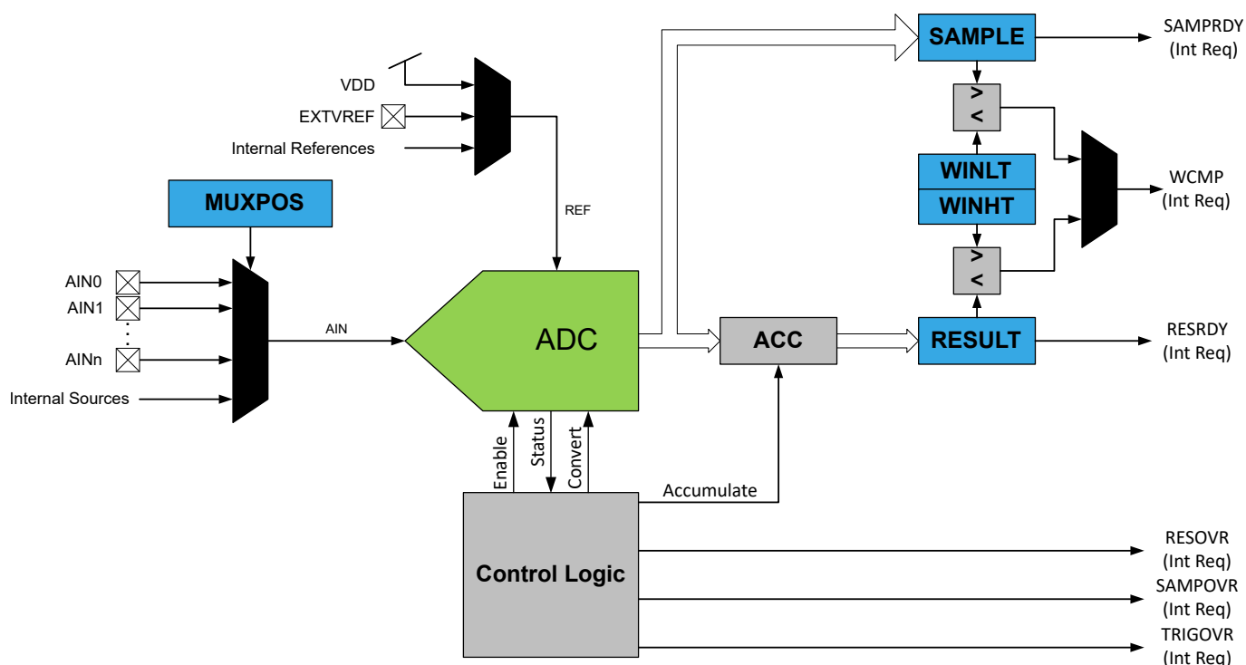
Figure 32-1. Block Diagram
