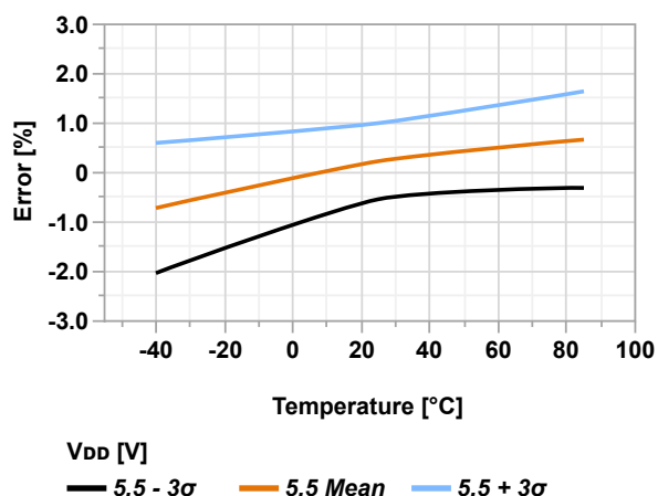
Figure 36-90. ACREF Voltage Error vs. Temperature ( V_{DD} = 5.5V , V_{VREF} = 2.048V )
