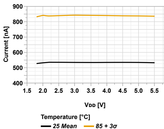
Figure 36-27. RTC Power Consumption vs. V_{DD}
