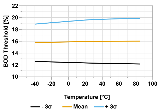
Figure 36-60. VLM Threshold vs. Temperature (VLMCTRL.VLMLVL = 0x02)
