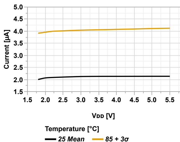
Figure 36-10. Idle Power Consumption vs. V_{DD} (MCLKCTRLA.CLKSEL = OSC32K)
