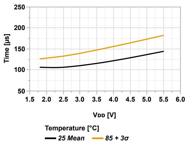
Figure 36-39. Wake-up Time from Power-Down vs. V_{DD} (OSCHF = 16 MHz, VREGCTRL = AUTO)
