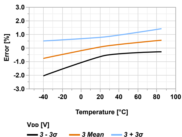
Figure 36-86. ADC0REF Voltage Error vs. Temperature ( V_{DD} = 3.0V , V_{VREF} = 2.5V )
