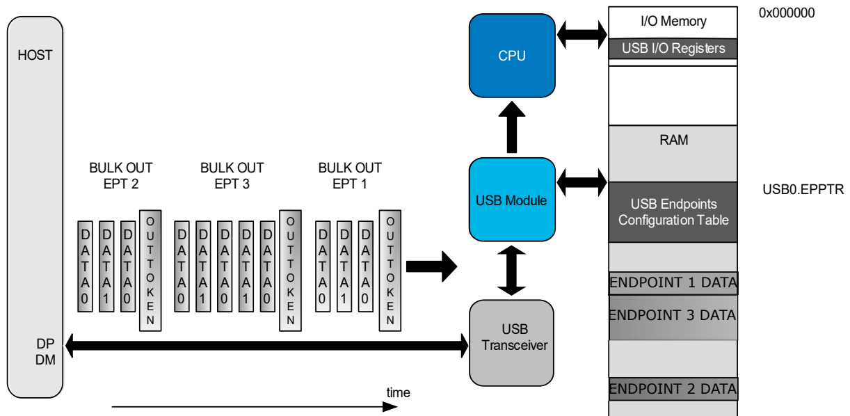
Figure 28-1. USB Out Transfer: Data Packet From Host To USB Device
