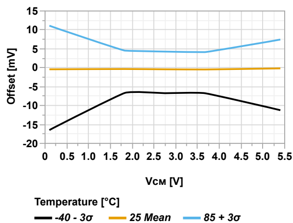
Figure 36-116. Input Offset vs. Common Mode Voltage ( V_{DD} = 5.5V )
