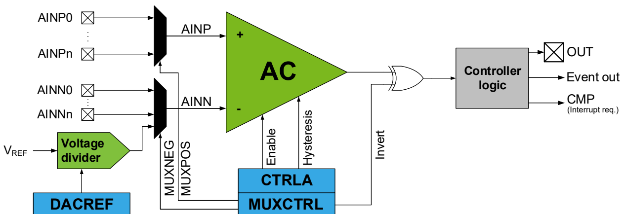
Figure 31-1. AC Block Diagram
