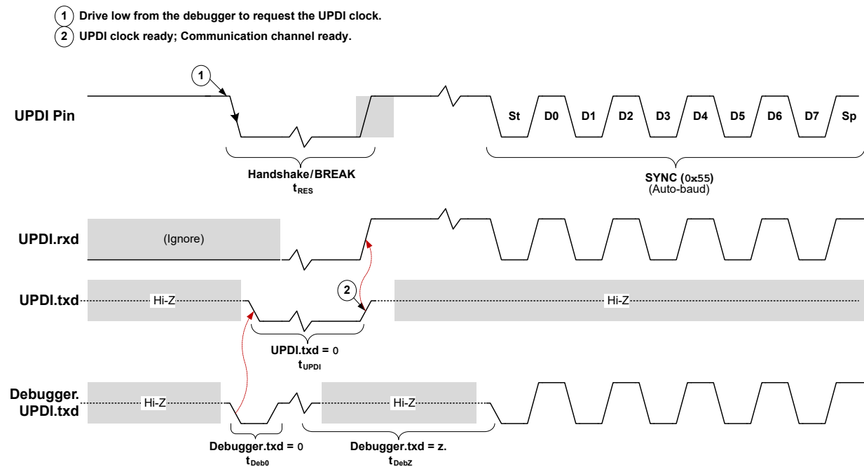
Figure 35-8. UPDI Enable Sequence with Dedicated UPDI Pin
