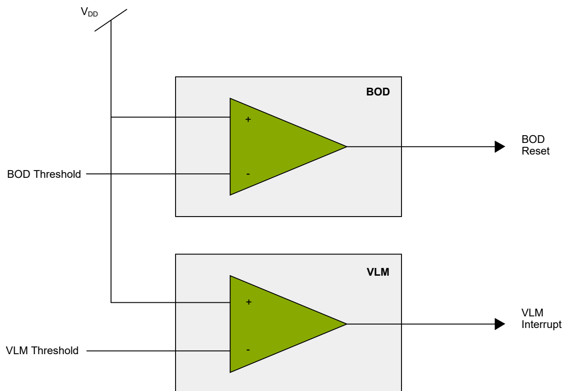
Figure 19-1. BOD Block Diagram
