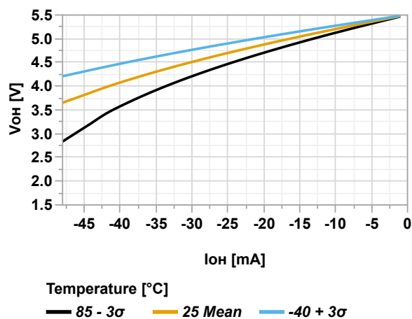
Figure 36-80. Output Pin - Minimum V_{OH} vs. Current, V_{DD} = 5.5V
