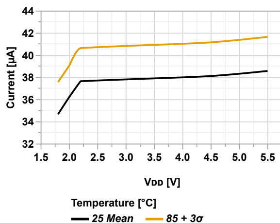
Figure 36-34. VREF Power Consumption vs. V_{DD} (ACREF Enabled)
