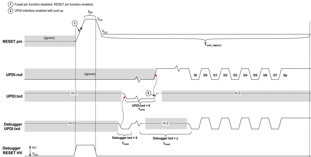
Figure 35-9. UPDI Enable Sequence by High-Voltage (HV) Programming
