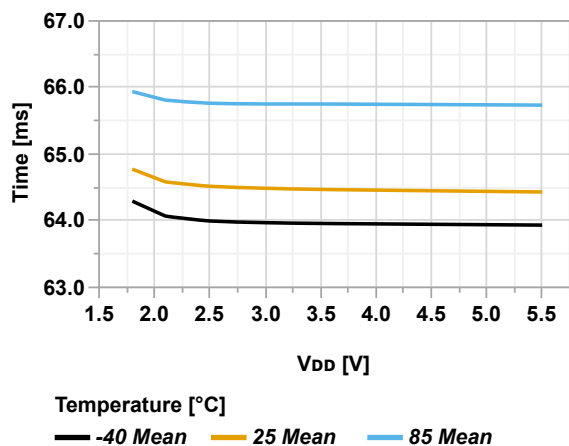
Figure 36-45. Start-up Time vs. V_{DD} (SYSCFG1 = 0x07)
