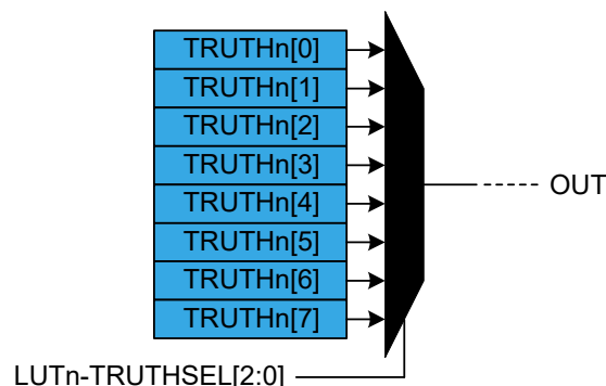
Figure 30-2. Truth Table Output Value Selection of an LUT
