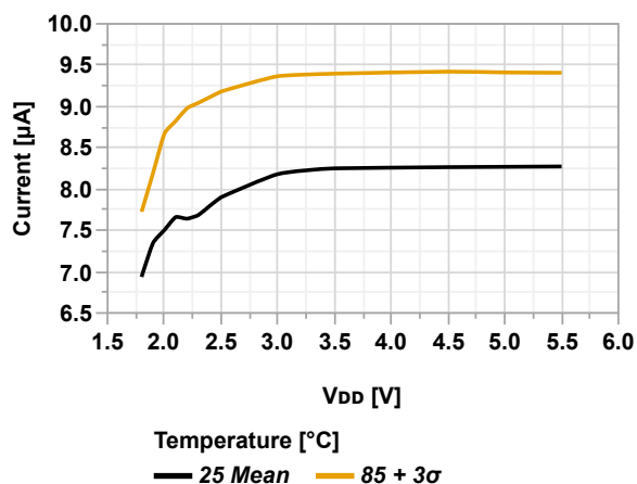
Figure 36-32. USART Power Consumption vs. V_{DD} (USART Enabled @9600 Baud)
