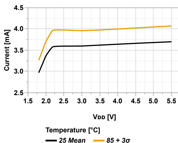
Figure 36-2. Active Power Consumption vs. V_{DD} (MCLKCTRLA.CLKSEL = EXTCLK, EXTCLK = 24 MHz)
