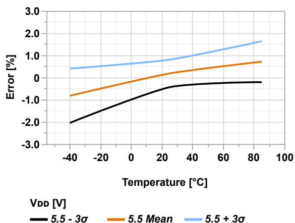
Figure 36-83. ADCOREF Voltage Error vs. Temperature ( V_{DD} = 5.5V , V_{VREF} = 2.048V )
