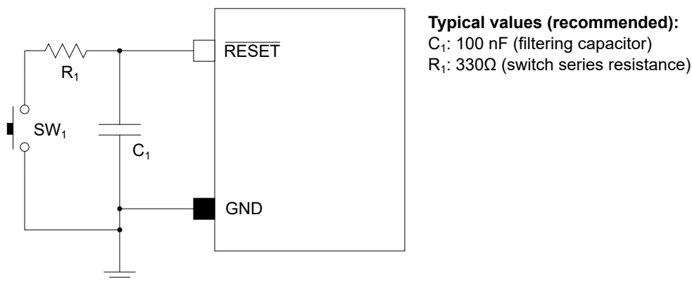
Figure 5-2. Recommended External Reset Circuit Schematic
