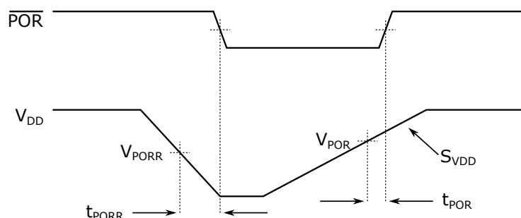
Figure 35-1. \overline{\text{POR}} and \overline{\text{PORR}} with Slow Rising V_{DD}
