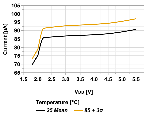
Figure 36-33. VREF Power Consumption vs. V_{DD} (ADCOREF Enabled)
