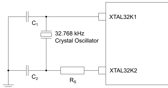
Figure 5-5. Recommended External 32.768 kHz Oscillator Connection Circuit Schematic
