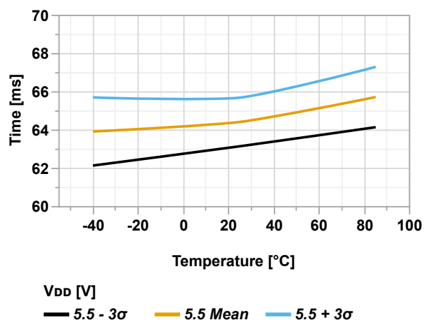
Figure 36-48. Start-up Time vs. Temperature (SYSCFG1 = 0x07, V_{DD} = 5.5V )
