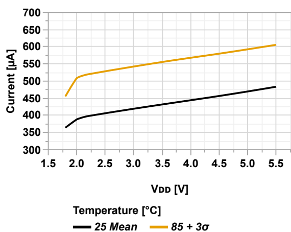
Figure 36-20. ADC Power Consumption vs. V_{DD} (ADC @85 kps)
