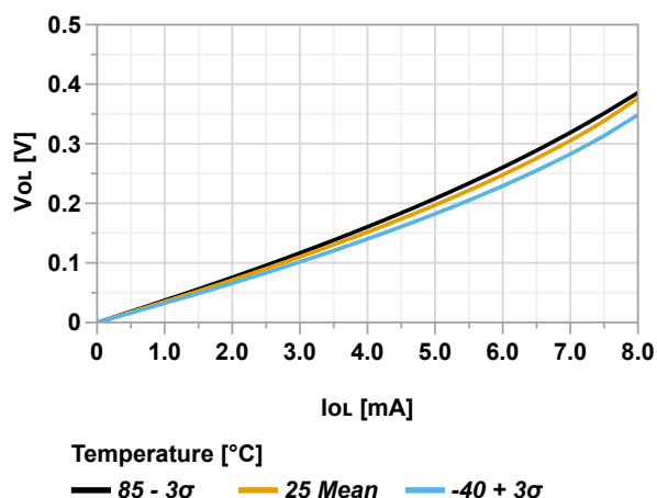
Figure 36-75. Output Pin - Maximum V_{OL} vs. Current, V_{DD} = 1.8V
