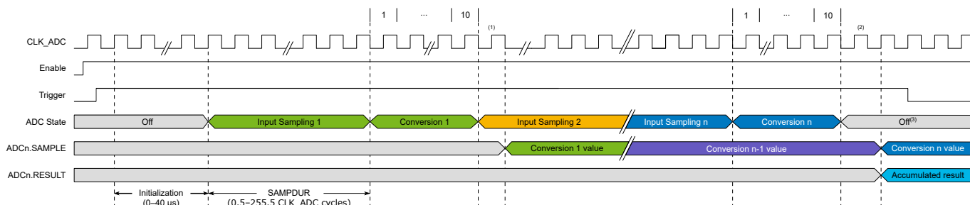
Figure 32-5. Timing Diagram - Burst Accumulation
