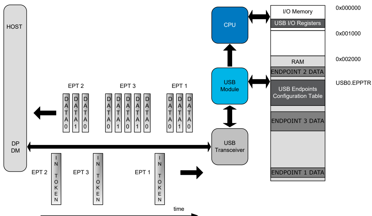
Figure 28-2. USB In Transfer: Data Packet From USB Device To Host After Request From Host
