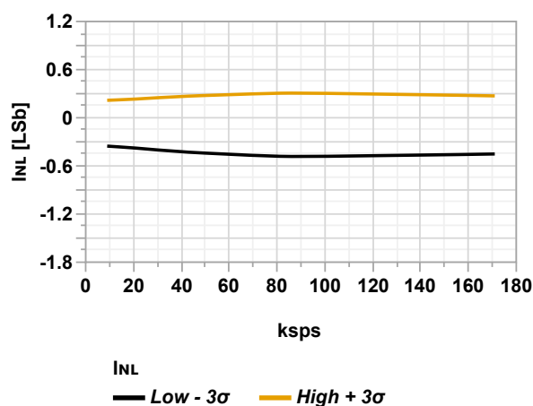
Figure 36-103. INL vs. Sample Rate (ADC Single Ended Mode, V_{REFA} = V_{DD} = 3.0V , T = 85^{\circ}C )
