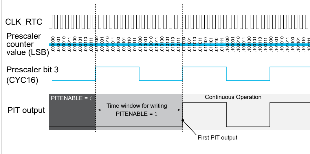
Figure 22-2. Timing Between PIT Enable and First Interrupt
