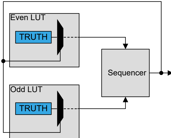
Figure 30-3. Feedback Input Selection
