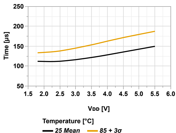
Figure 36-43. Wake-up Time from Power-Down vs. V_{DD} (OSC32K, VREGCTRL = AUTO)
