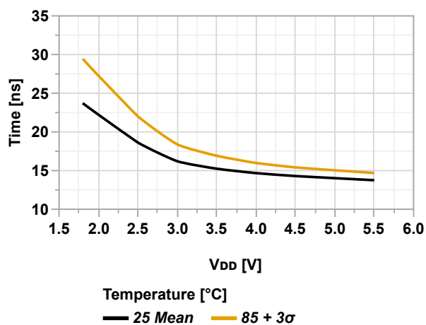
Figure 36-64. Rise Time vs. V_{DD} (PORTCTRL.SRL = 0x00)
