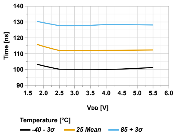
Figure 36-44. Minimum Reset Pulse Width vs. V_{DD}
