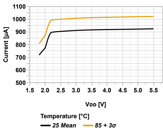
Figure 36-3. Active Power Consumption vs. V_{DD} (MCLKCTRLA.CLKSEL = OSCHF, OSCHF = 4 MHz)
