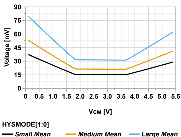
Figure 36-117. Input Hysteresis vs. Common Mode Voltage ( V_{DD} = 5.5V )
