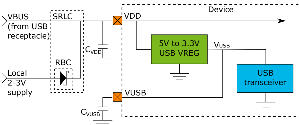
Figure 6-6. Power Configuration 5b2s
