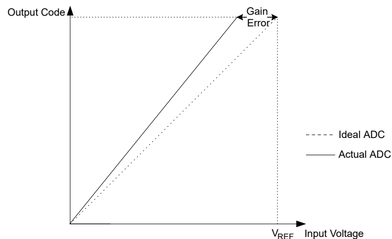
Figure 4-2. Gain Error
