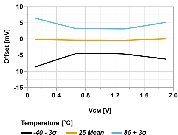
Figure 36-114. Input Offset vs. Common Mode Voltage ( V_{DD} = 3.0V )
