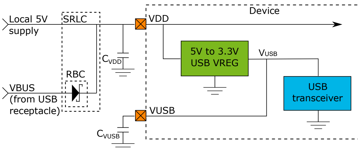
Figure 6-7. Power Configuration 5s5b
