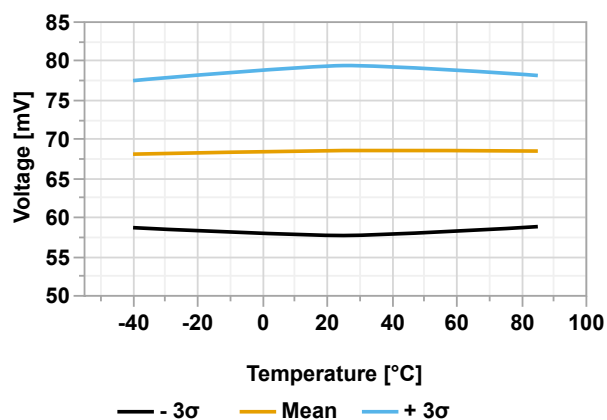
Figure 36-58. BOD Hysteresis vs. Temperature (BODCFG.LVL = 0x03)
