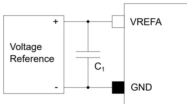
Figure 5-7. Recommended External Voltage Reference Connection
