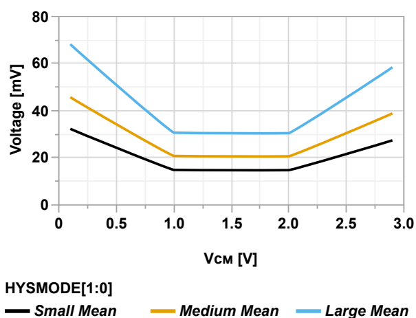
Figure 36-115. Input Hysteresis vs. Common Mode Voltage ( V_{DD} = 3.0V )
