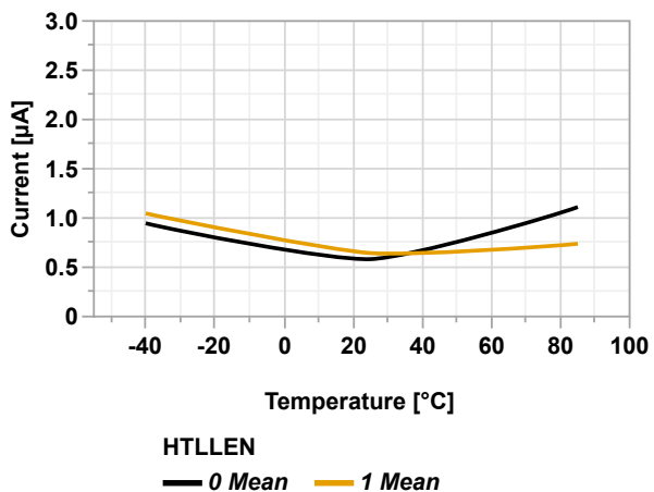
Figure 36-14. Typical +3 \sigma Power-Down Power Consumption vs. Temperature ( V_{DD} = 3.0V )
