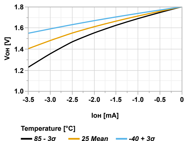
Figure 36-76. Output Pin - Minimum V_{OH} vs. Current, V_{DD} = 1.8V
