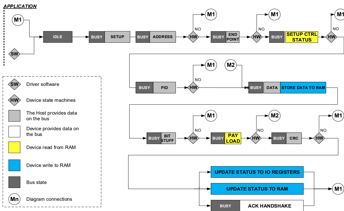
Figure 28-4. SETUP Transaction
