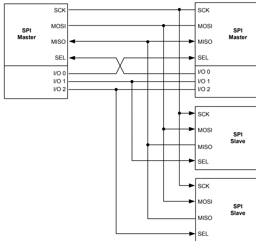
Figure 112. SPI Multi-Master Slave Environment
