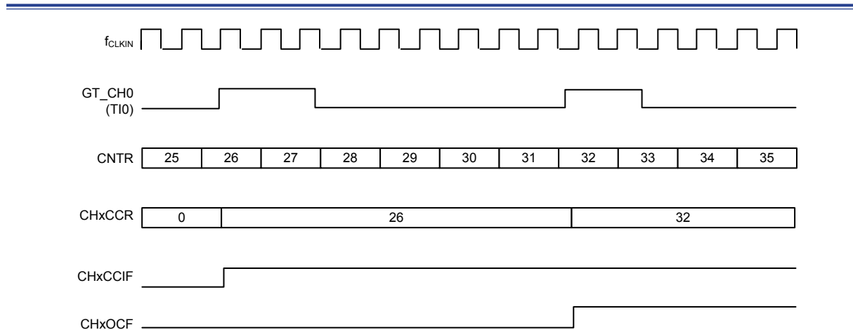
Figure 44. Input Capture Mode
