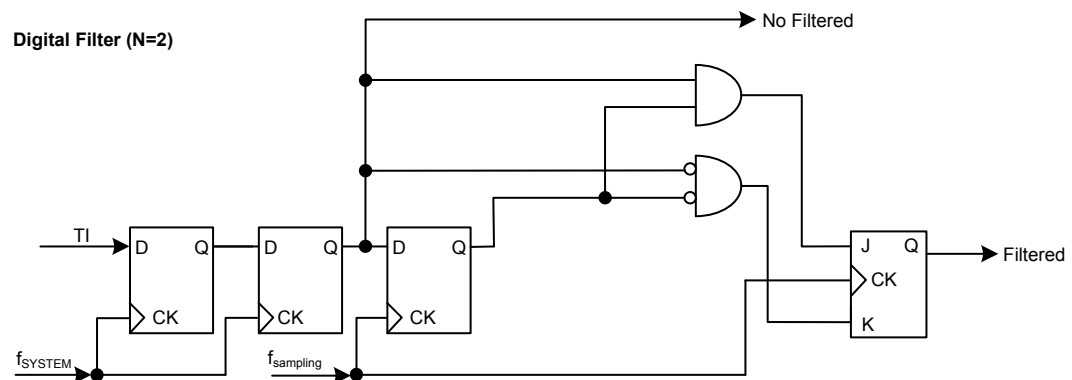
Figure 80. TI Digital Filter Diagram with N = 2
