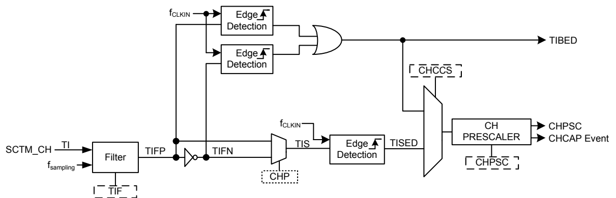
Figure 79. Channel Input Stages
