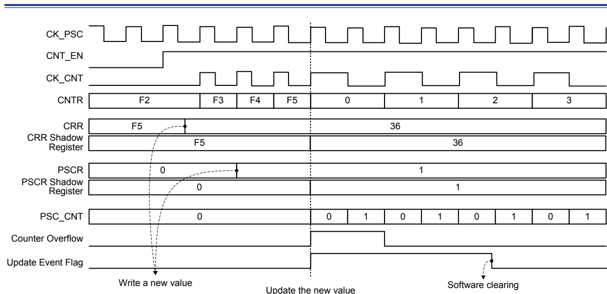
Figure 32. Up-counting Example
