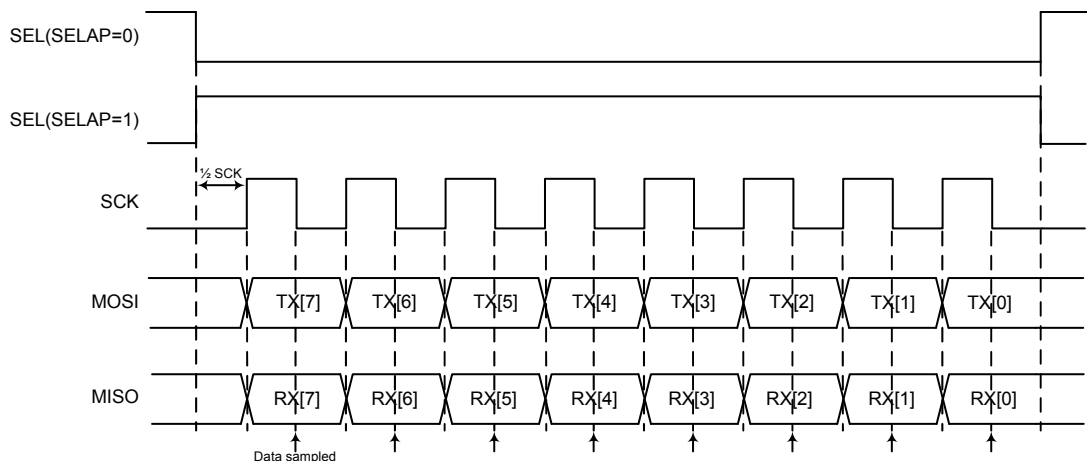
Figure 106. SPI Single Byte Transfer Timing Diagram – CPOL = 0, CPHA = 1
