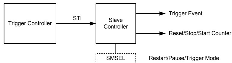
Figure 73. Slave Controller Diagram
