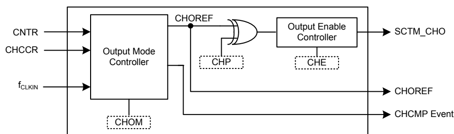
Figure 81. Output Stage Block Diagram
