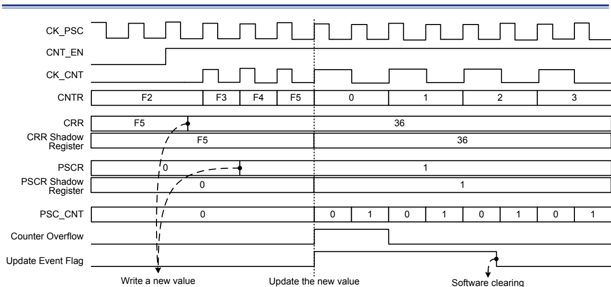
Figure 70. Up-counting Example
