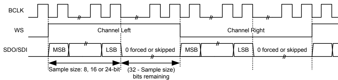
Figure 160. Left-justified Stereo Mode Waveforms (32-bit Channel Enabled)
