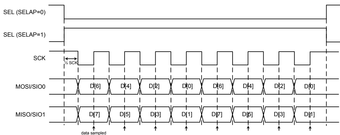
Figure 123. QSPI Dual Mode Bit Sequence – CPOL = 1, CPHA = 1, DFL = 0x8 (16-bit Data in total)
