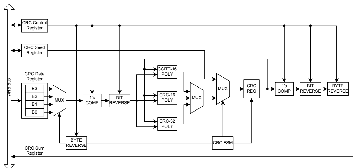
Figure 176. CRC Block Diagram
