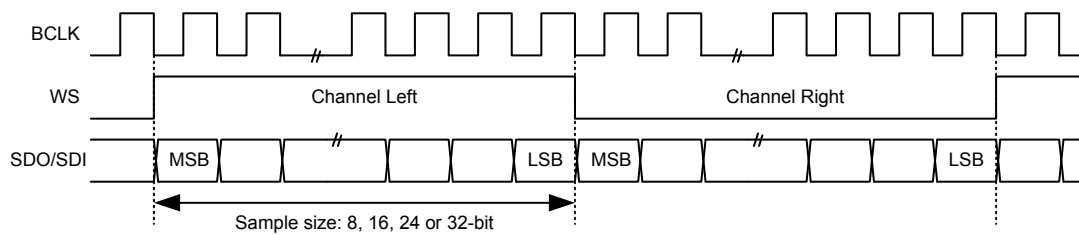
Figure 159. Left-justified Stereo Mode Waveforms
