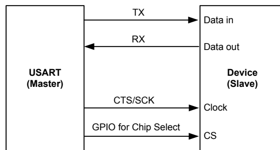
Figure 143. USART Synchronous Transmission Example
