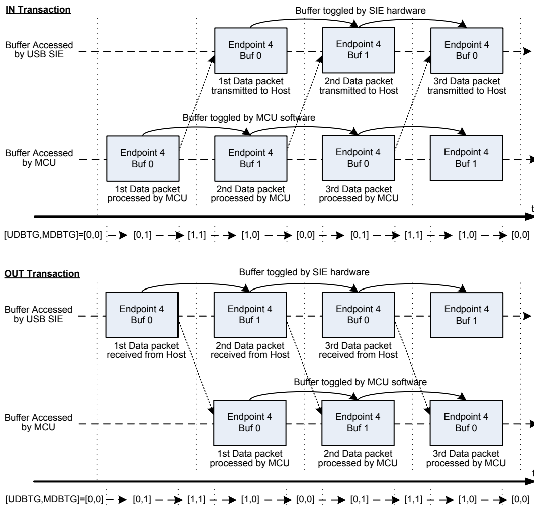
Figure 150. Double-buffering Operation Example
