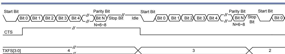
Figure 139. USART CTS Flow Control
