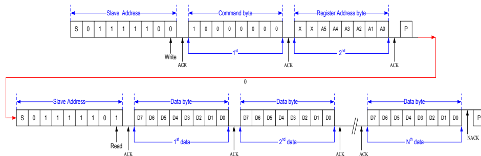
I²C Interface N Bytes Display RAM Data Read Operation
