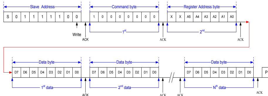
I²C Interface N Bytes Display RAM Data Write Operation
